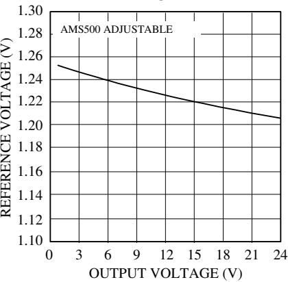
Reference Voltage
