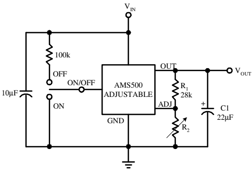
Typical application circuit (adjustable output)
