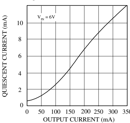
Quiescent Current
