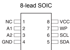
8-lead dBGGA2
