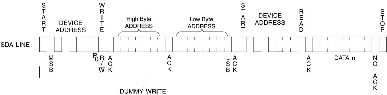
Figure 7-5. Random Read
