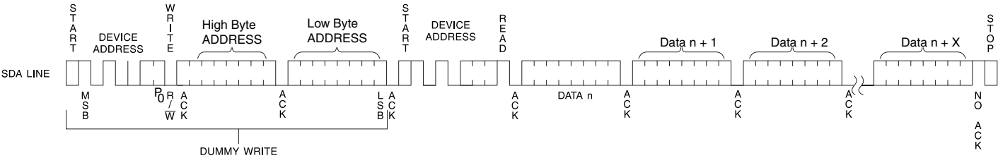
Figure 7-6. Sequential Read
