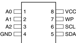
8-lead SOIC
