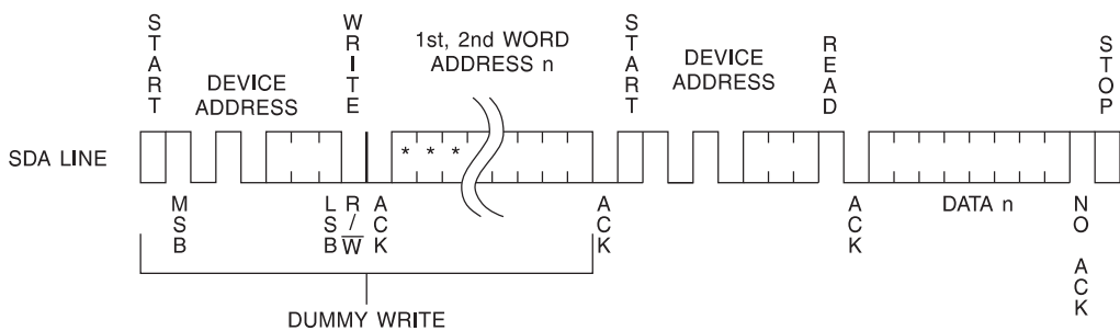
Figure 11. Random Read
