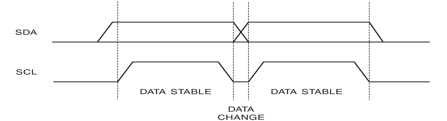
Figure 4. Data Validity
