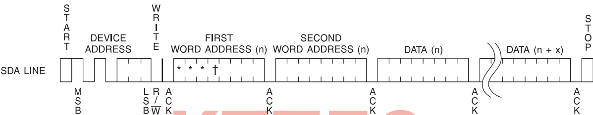
Figure 9. Page Write
