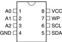
8-lead TSSOP
