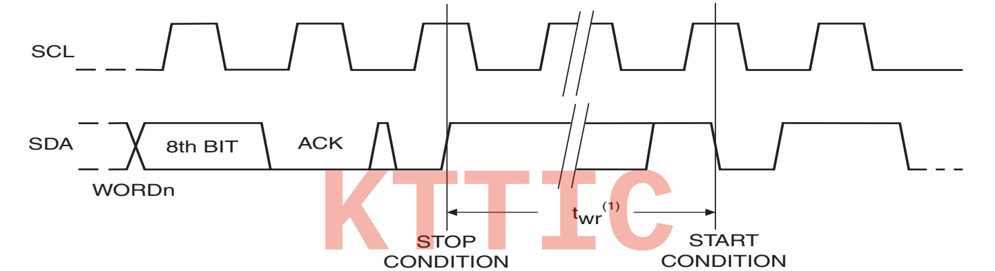
Figure 3. Write Cycle Timing SCL: Serial Clock, SDA: Serial Data I/O
