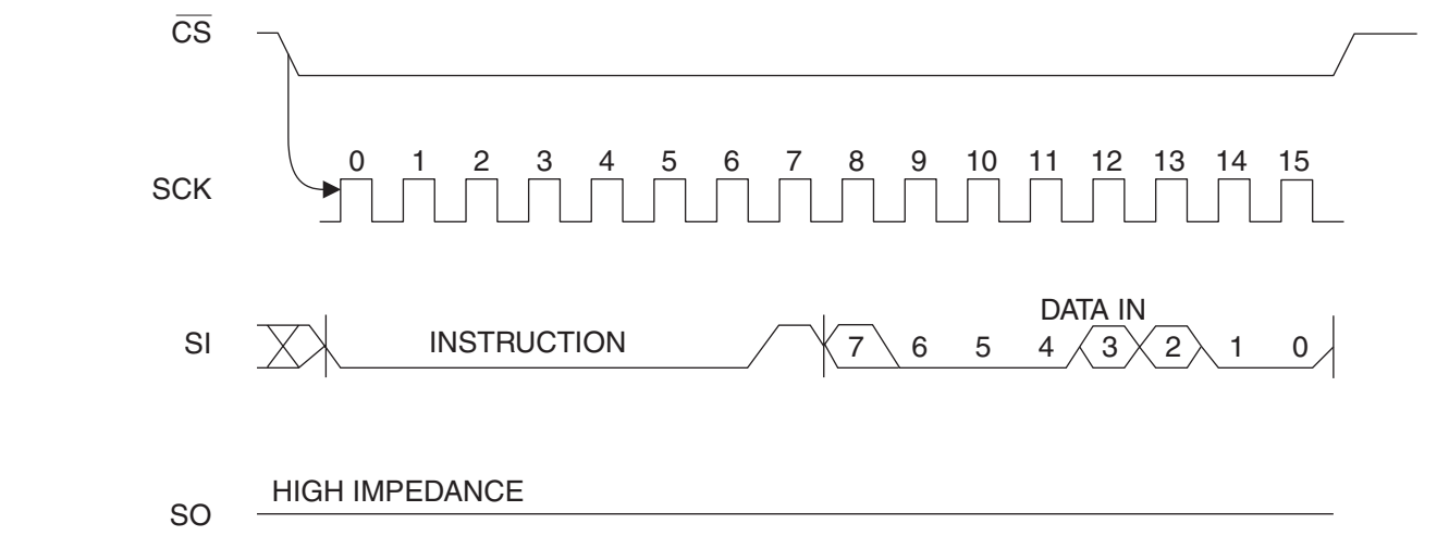
Figure 4-5. WRSR Timing
