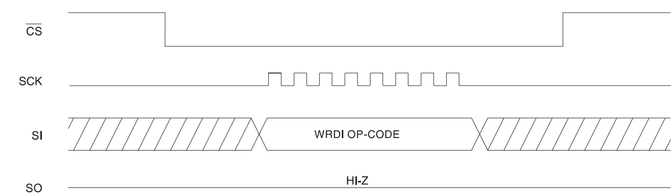
Figure 4-3. WRDI Timing
