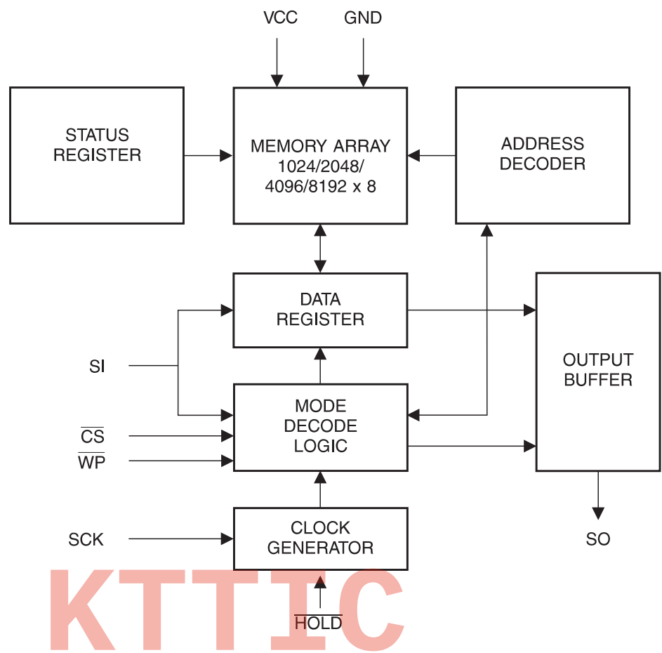
Figure 1-1. Block Diagram
