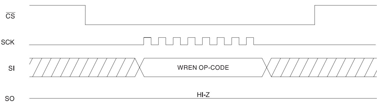
Figure 4-2. WREN Timing
