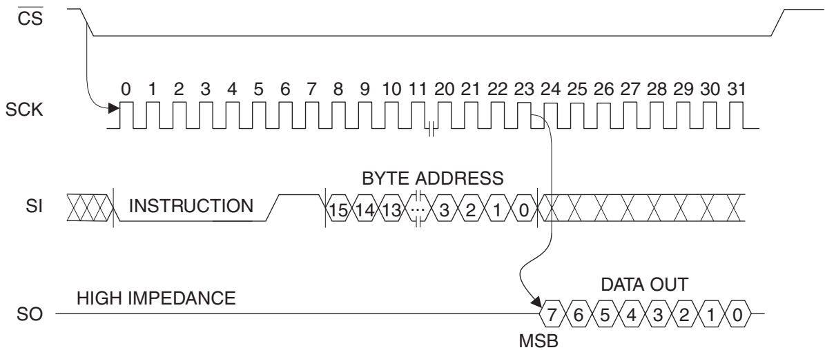
Figure 4-6. READ Timing
