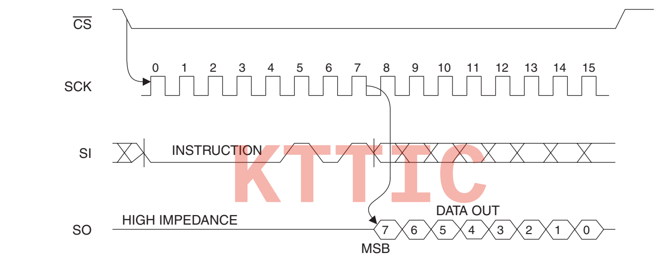
Figure 4-4. RDSR Timing
