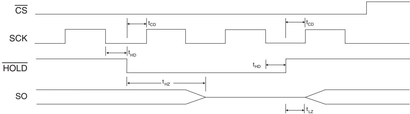
Figure 4-8. \overline{HOLD} Timing
