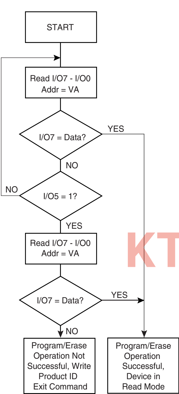
Figure 4-1. Data Polling Algorithm (Configuration Register = 00)
