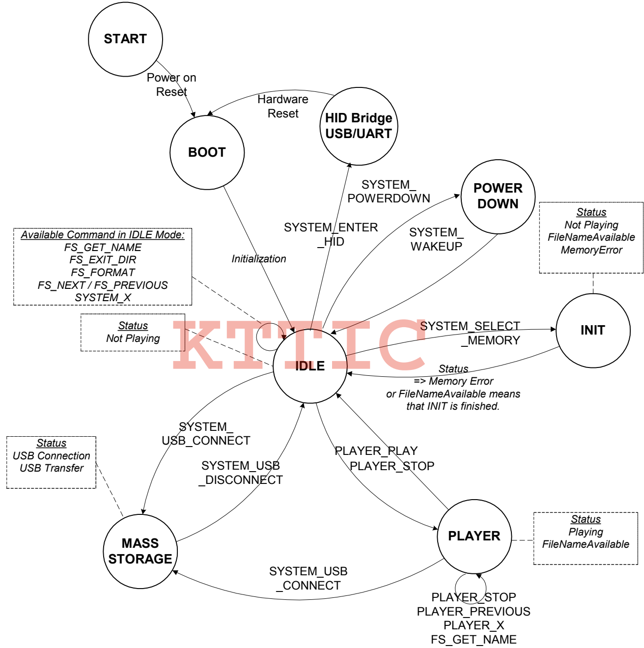
Figure 3-2. Player's Operating Modes
