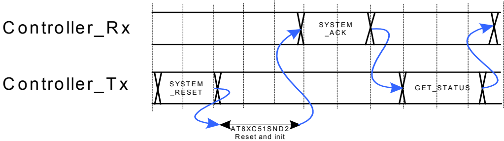
Figure 3-4 . Warm Reset
