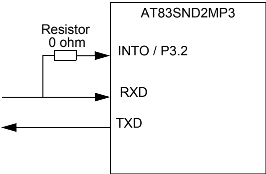
Figure 5-1 . AT83SND2CMP3 Configuration for SYSTEM_WAKEUP Command
