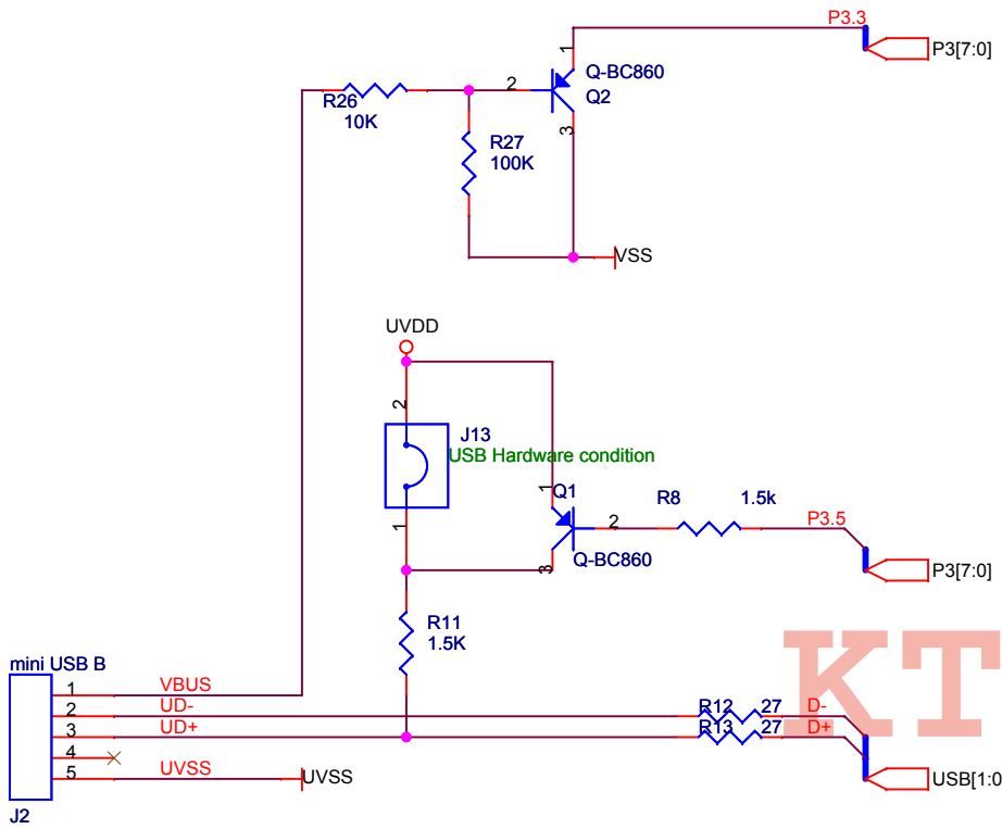
USB interface
