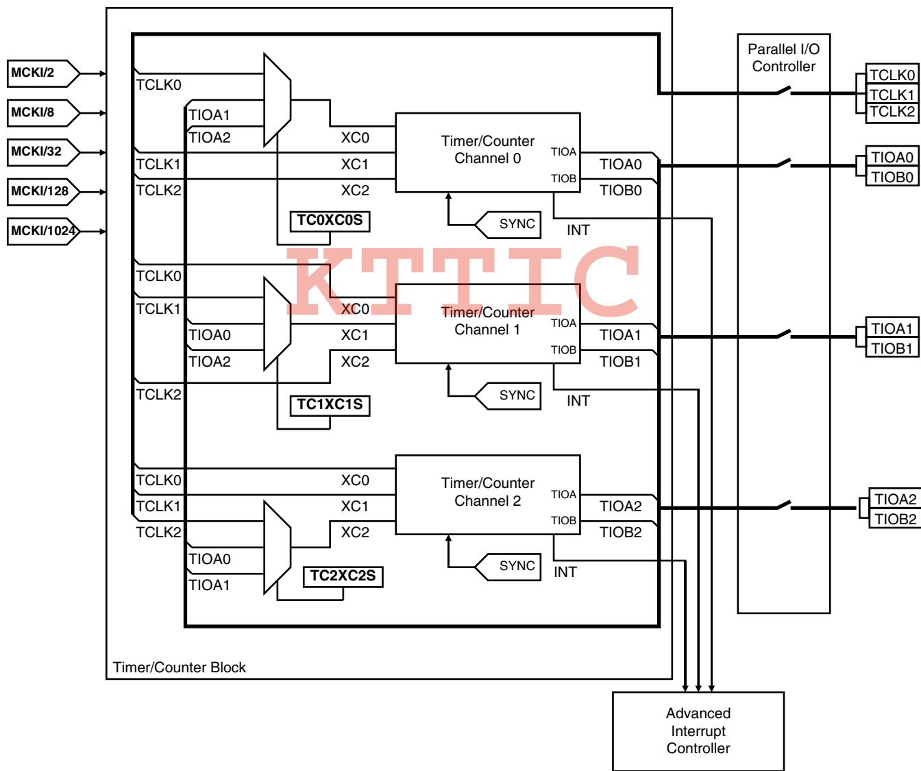
Figure 53. TC Block Diagram
