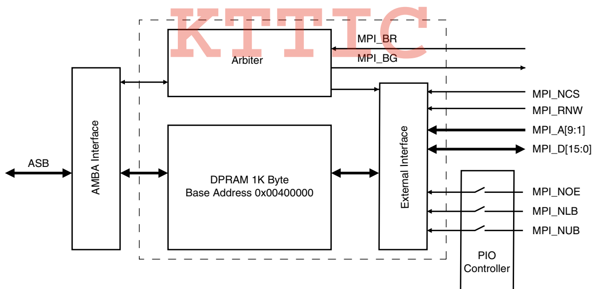
Figure 32. MPI Block Diagram
