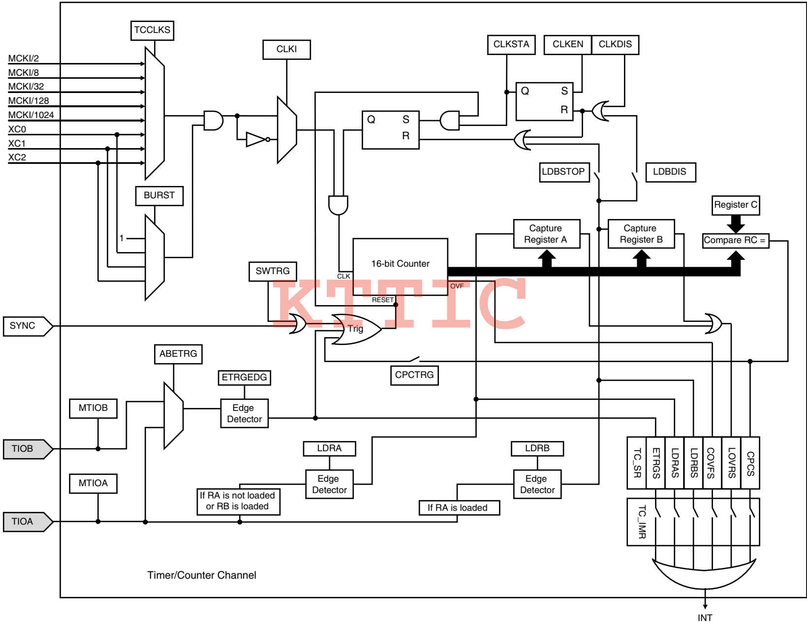
Figure 56. Capture Mode
