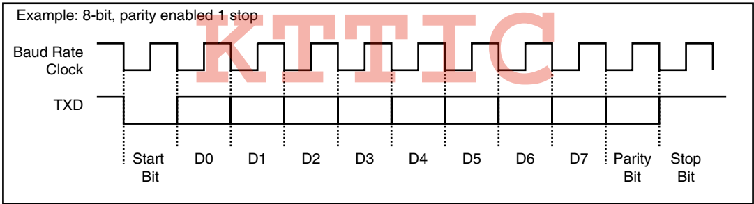
Figure 44. Synchronous and Asynchronous Modes: Character Transmission
