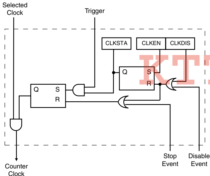
Figure 55. Clock Control
