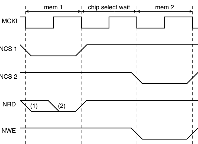
Figure 20. Chip Select Wait
