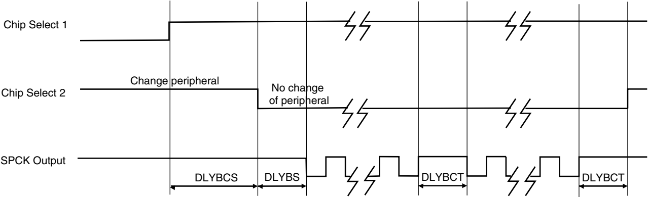
Figure 52. Programmable Delays (DLYBCS, DLYBS and DLYBCT)
