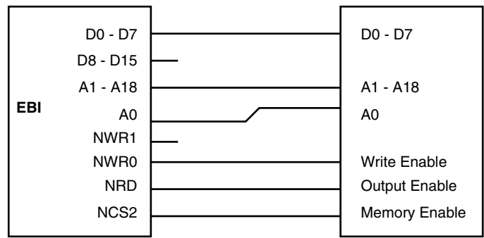
Figure 8. Memory Connection for an 8-bit Data Bus
