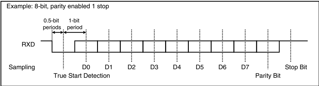
Figure 42. Asynchronous Mode: Character Reception
