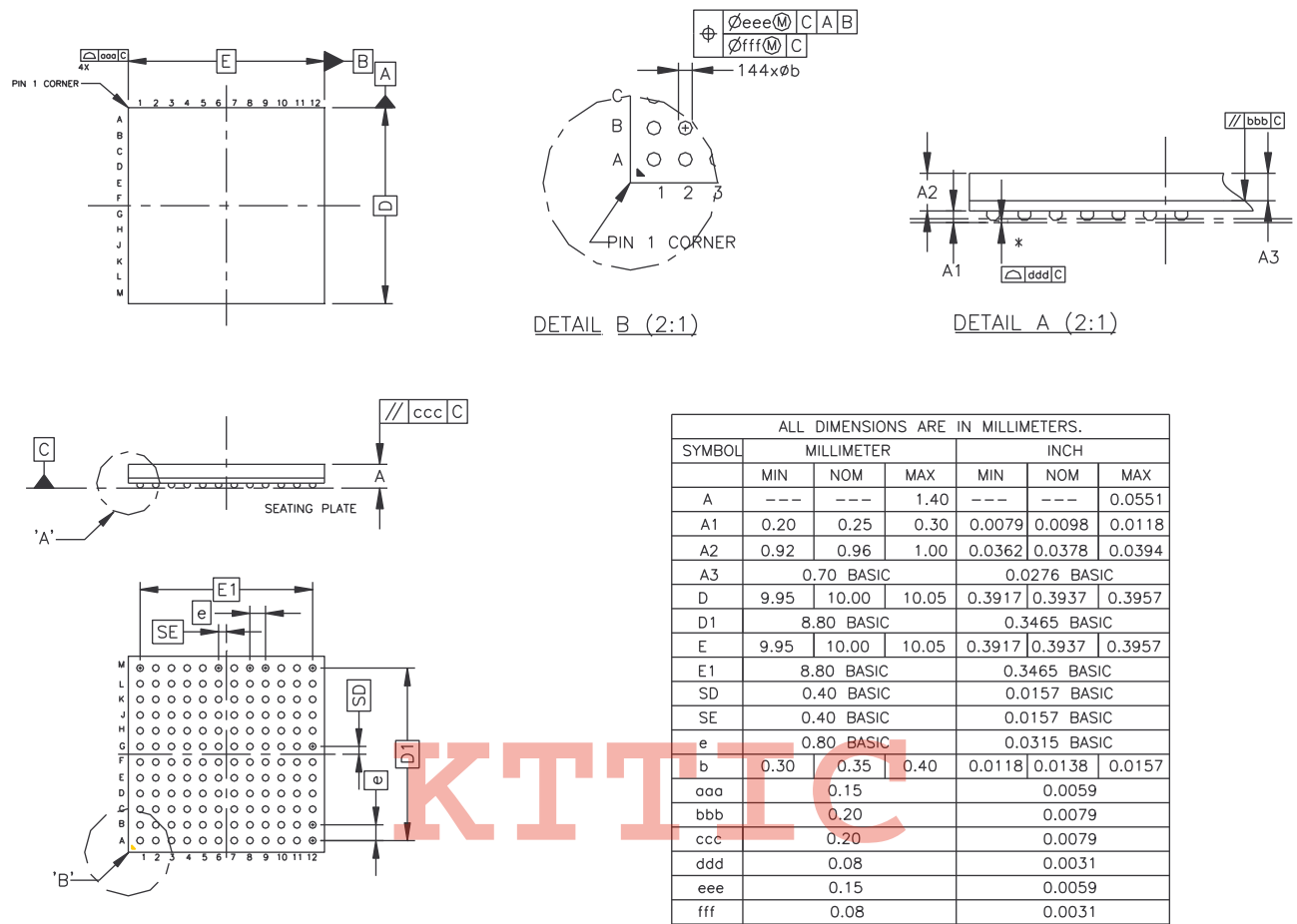
Figure 12-1. 144-ball LFBGA Package Drawing
