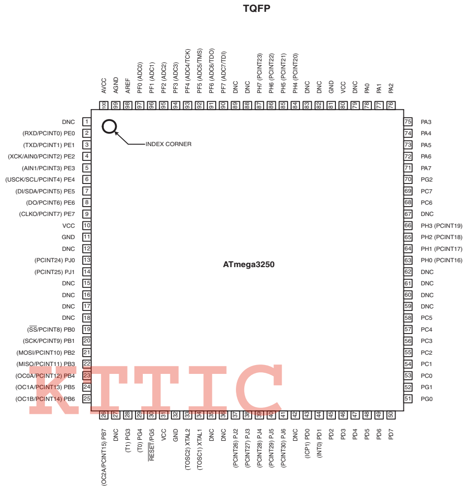
Figure 1-1. Pinout ATmega3250P
