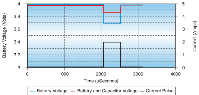
Figure 5. GSM Pulse
