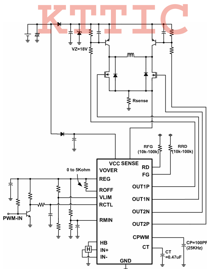
Figure 1. 12V Application Circuit
