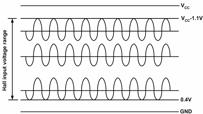
Figure 3. Hall input voltage range
