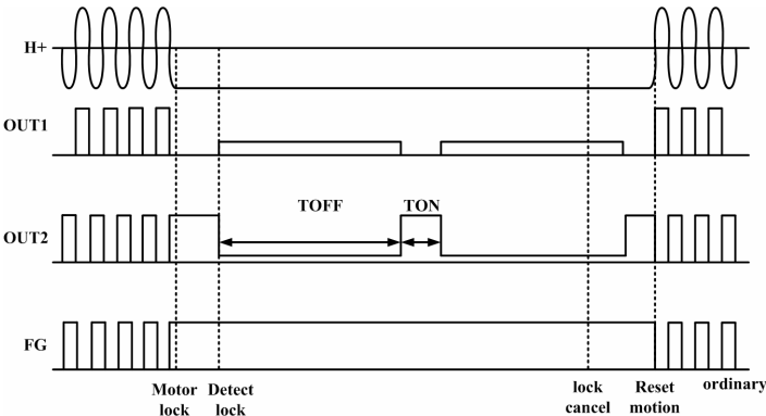
Figure 7. Lock detect and auto restart motion
