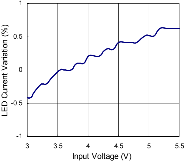
LED Current Regulation (10mA)
