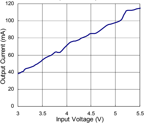
Maximum Output Current vs. Input Voltage (10WLEDs)
