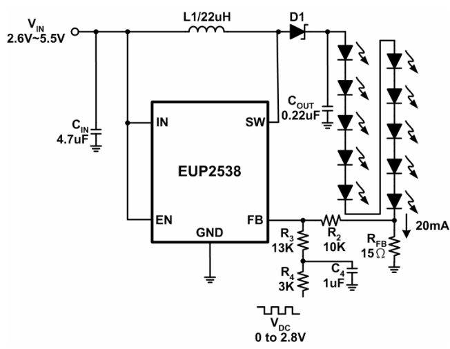
Figure 6. Filtered PWM Dimming Control
