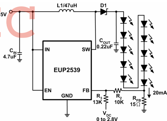
Figure 5. DC Voltage Dimming Control
