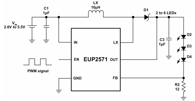
Figure 4. PWM Dimming Control Using the EN Pin
