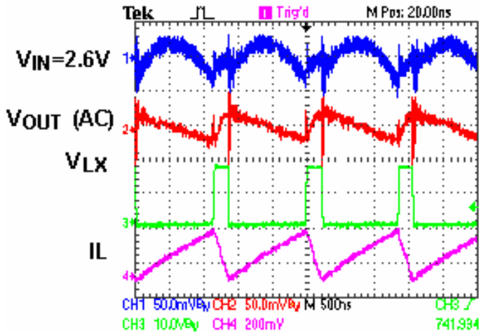
Stability for Driving 5 WLEDs
