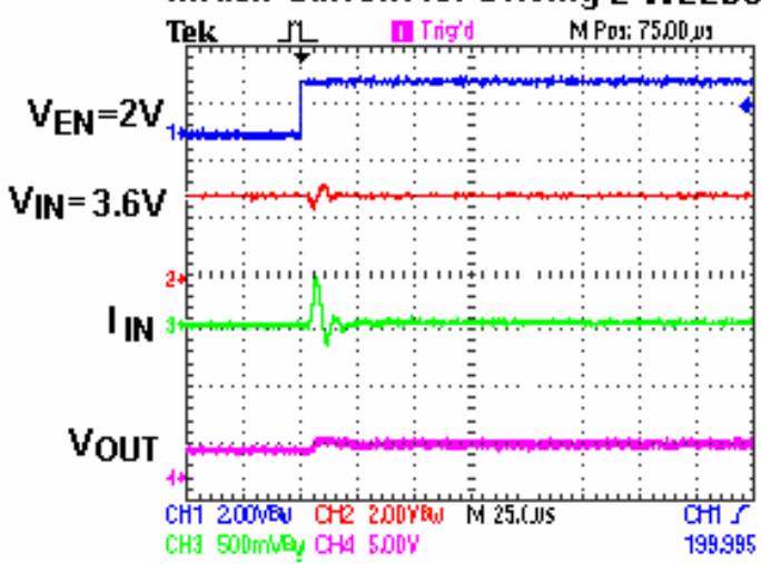
Inrush Current for Driving 2 WLEDs
