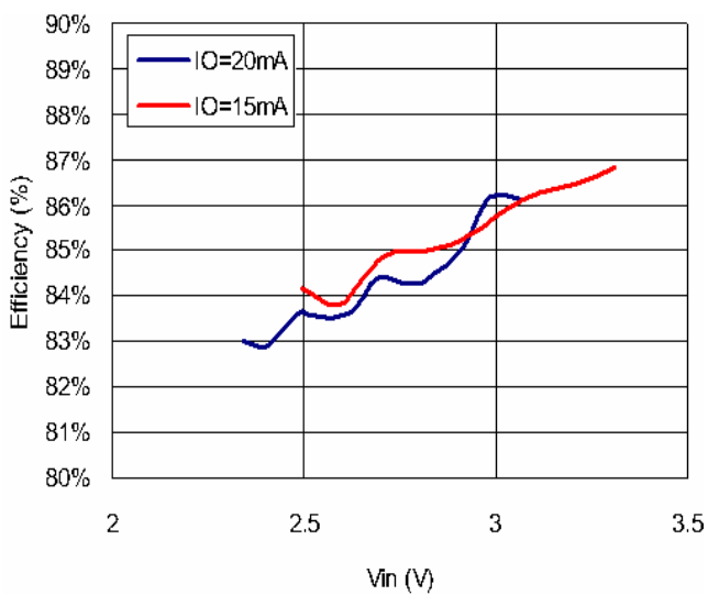
Efficiency vs. Vin (Driving 1WLED)
