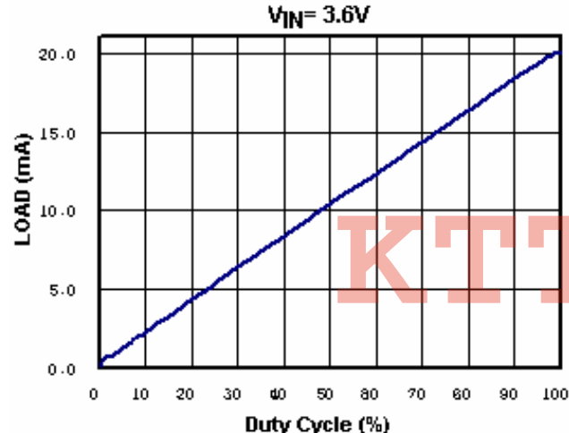
Duty Cycle vs. Load Current (PWM at EN)
