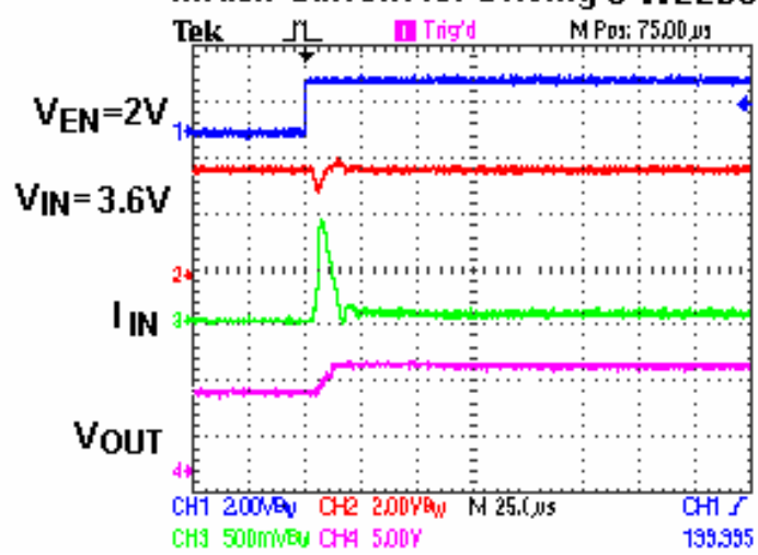
Inrush Current for Driving 3 WLEDs
