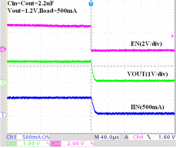
Turn Off Waveforms
