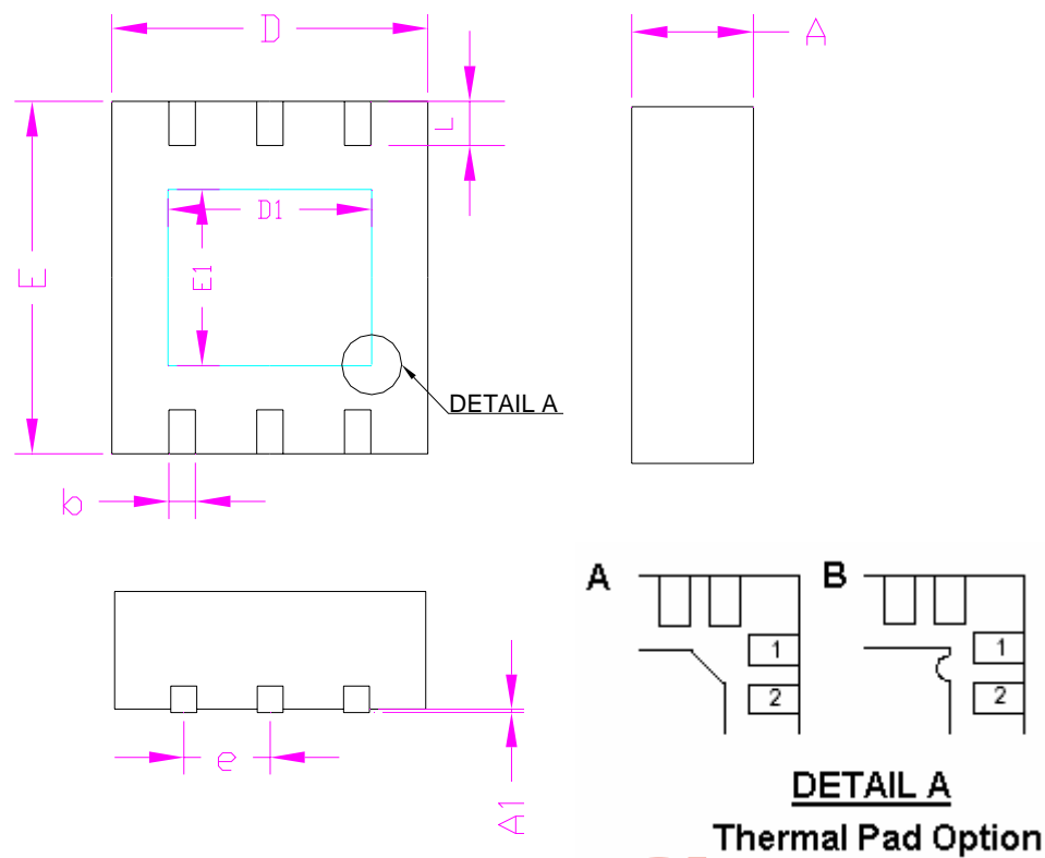
TDFN-6
