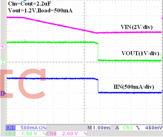
Power Off Waveforms
