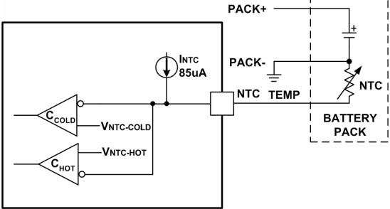
Figure 7. Temperature Sensing Configuration
