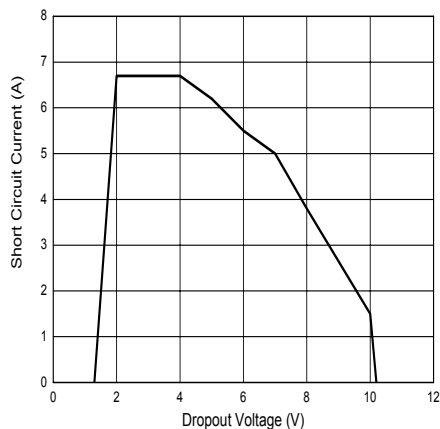
Figure 9. Short Circuit Current vs. Dropout Voltage
