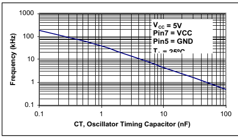
Figure 3. Oscillator Frequency vs. Timing Capacitor
