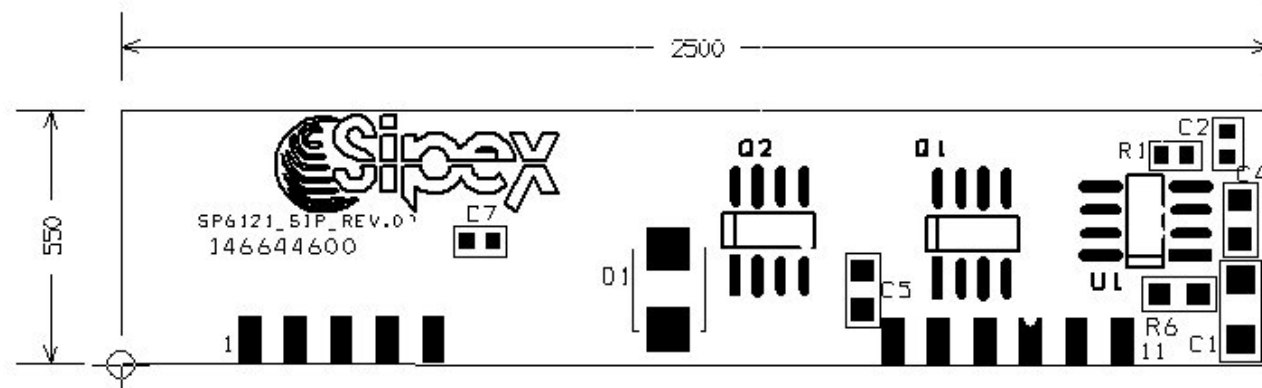
FIGURE 1. SP6121 Demo Board – layer 1, top view.
