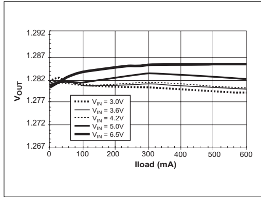
Figure 8. Line/Load Rejection, V_{OUT} = 1.25V , LI = 22\mu H (Sumida CDRH6D28), I_{LM} = V_{IN}
