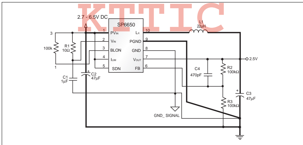
Figure 21. Application circuit with highlighted power traces.
