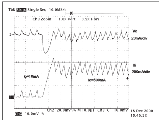
Figure 12. Load Step Transient Response, V_{OUT} = 2.5V , 10mA to 500mA. LI = 22\mu H (Sumida CDRH6D28), I_{LM} = V_{IN}
