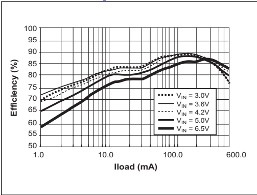
Figure 7. Efficiency vs. Output Current, V_{OUT} = 1.25V , LI = 22\mu H (Sumida CDRH6D28), I_{LM} = V_{IN}
