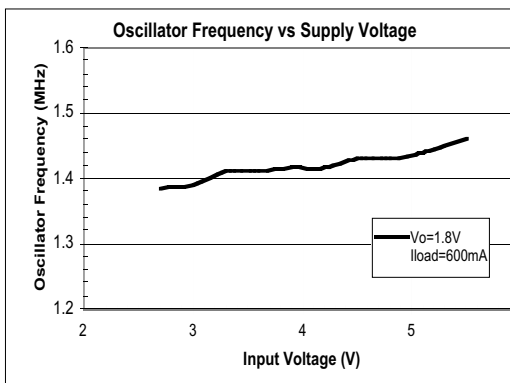
Figure 12: Oscillator Frequency vs. Supply Voltage
