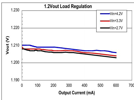
Figure 18: Load Regulation V_{out} = 1.2V
