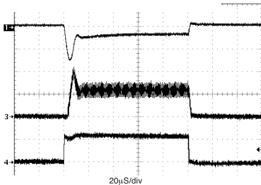
Figure 1: Load Transient 0mA to 600mA
