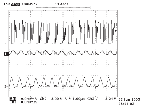
Figure 21. SP6659 Idle Mode Operation
