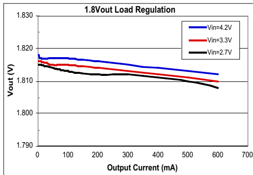
Figure 8: Load Regulation V_{out} = 1.8V
