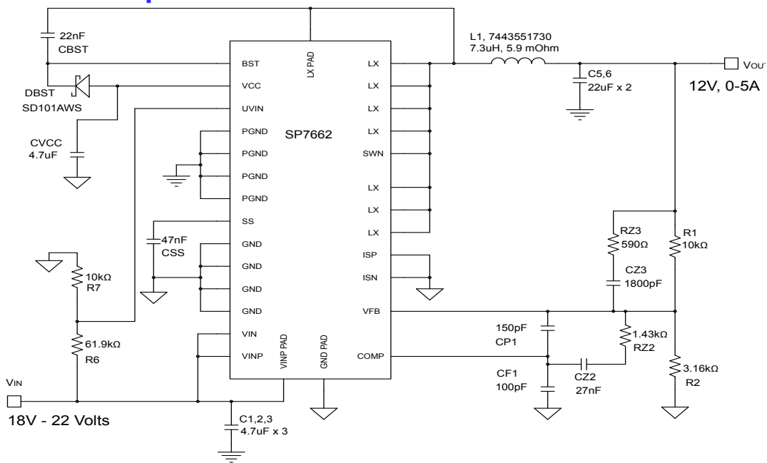
SP7662 with 12 VOUT (>3.3Volts) configuration
