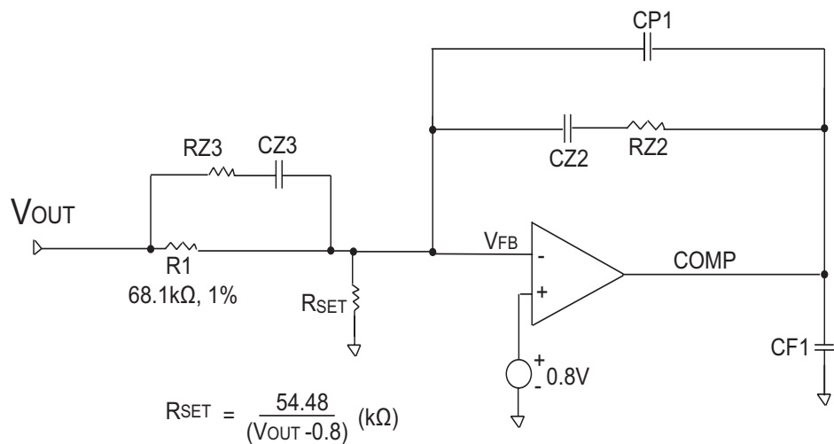
Type III Error Amplifier Compensation Circuit
