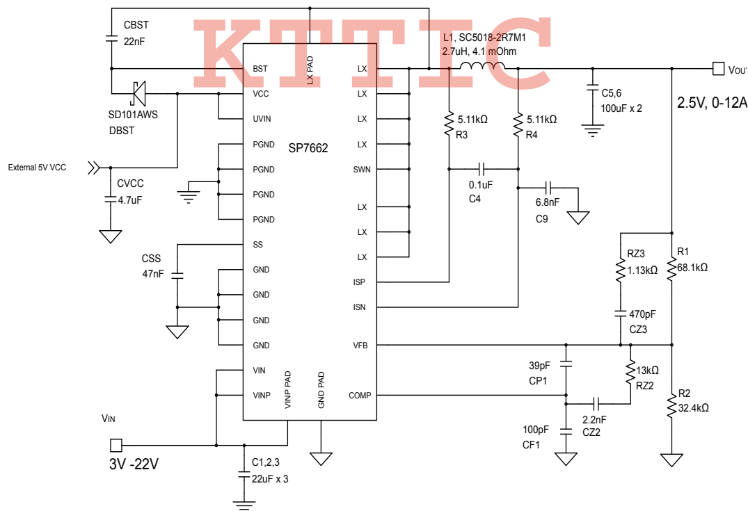
SP7662 with 3 to 22V input configuration
