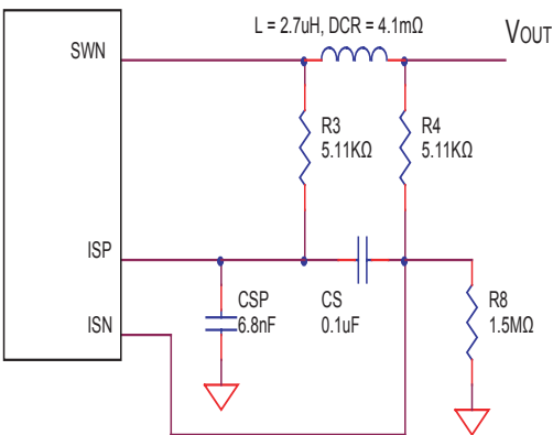
Over-current detection circuit for I_{\text{MAX}} < \{60\text{mV} / \text{DCR}\}
