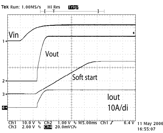
Start up response, Iout=12A
