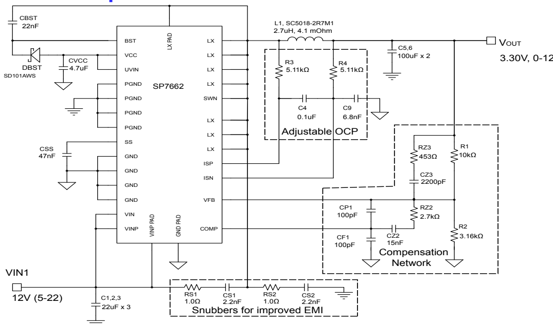
Typical Schematic showing circuit function blocks. Efficiency data was produced using this circuit.
