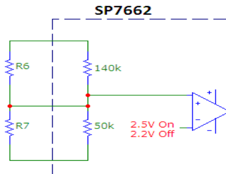
Internal and external bias of UVIN
