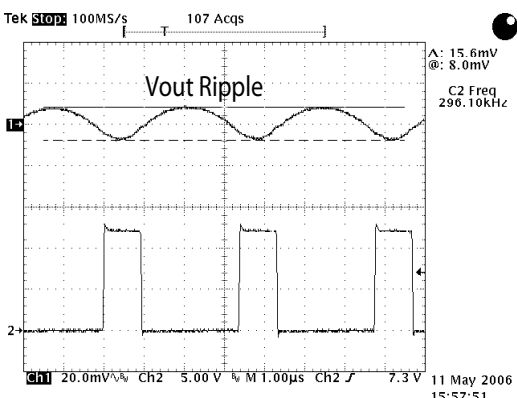
Output Ripple, No Load
