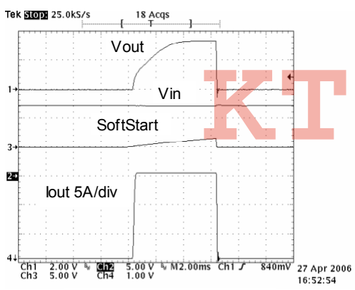
OCP Hiccup Response
