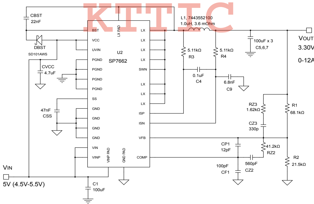
SP7662 with 4.5 to 5.5Vin configuration
