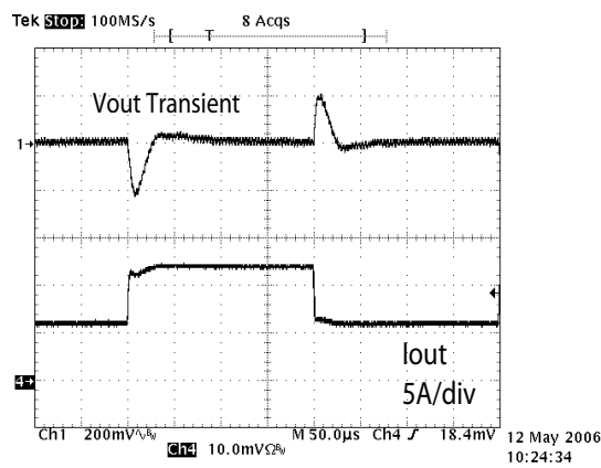
Load Step Response, Iout=6A -12A
