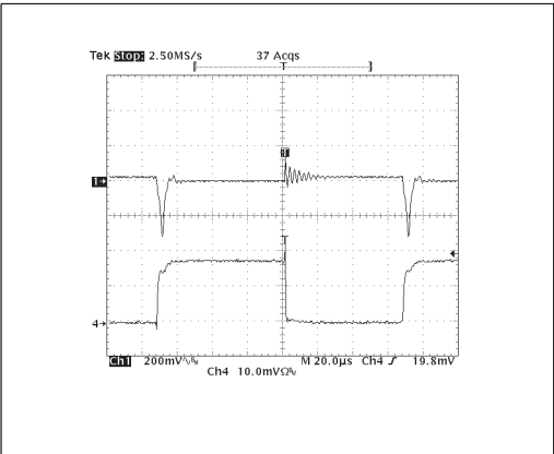
Figure 17. Load Step Response (0 to 800mA), Vin=3.3V, Vout=1.8V, Cin=10μF, Cout=2.2μF, OSCON; 1 = Vout, 4= Iload
