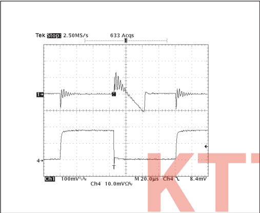
Figure 16. Load Step Response (0 to 800mA), Vin=3.3V, Vout=1.8V, Cin=10μF, Cout=2.2μF, Ceramic; 1 = Vout, 4= Iload
