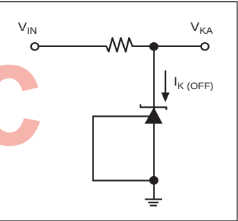
Figure 4. Test Circuit for I_{K(OFF)}
