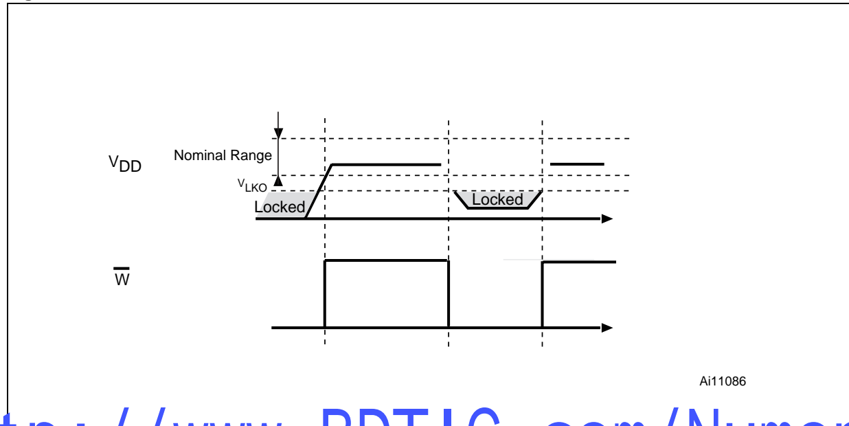
Figure 36. Data Protection
