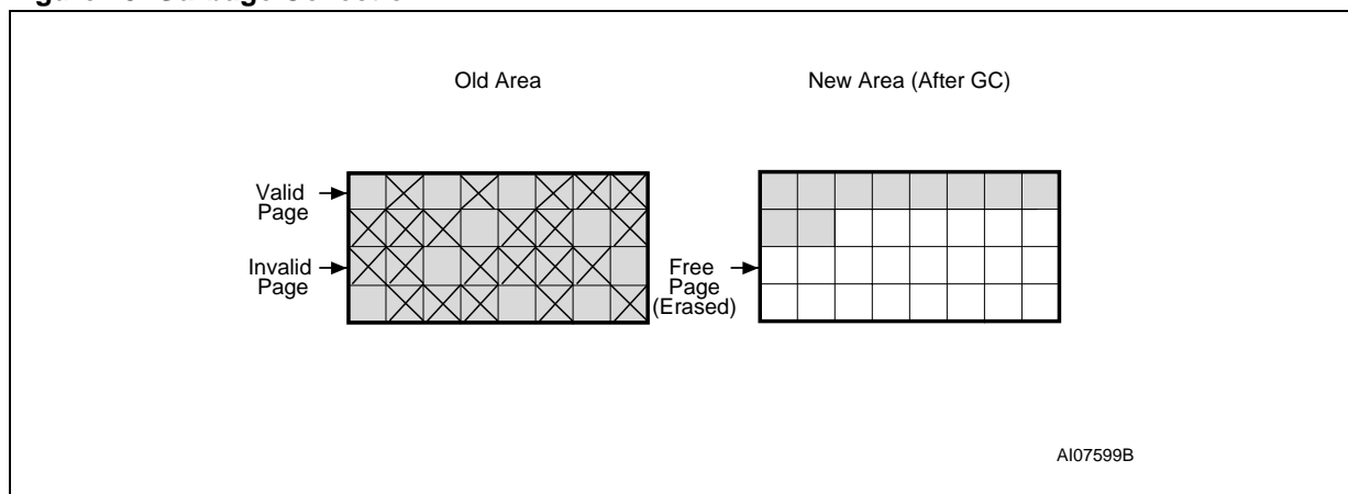
Figure 19. Garbage Collection
