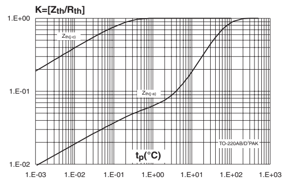
Figure 8: Relative variation of thermal impedance versus pulse duration (TO-220AB / D 2 PAK)
