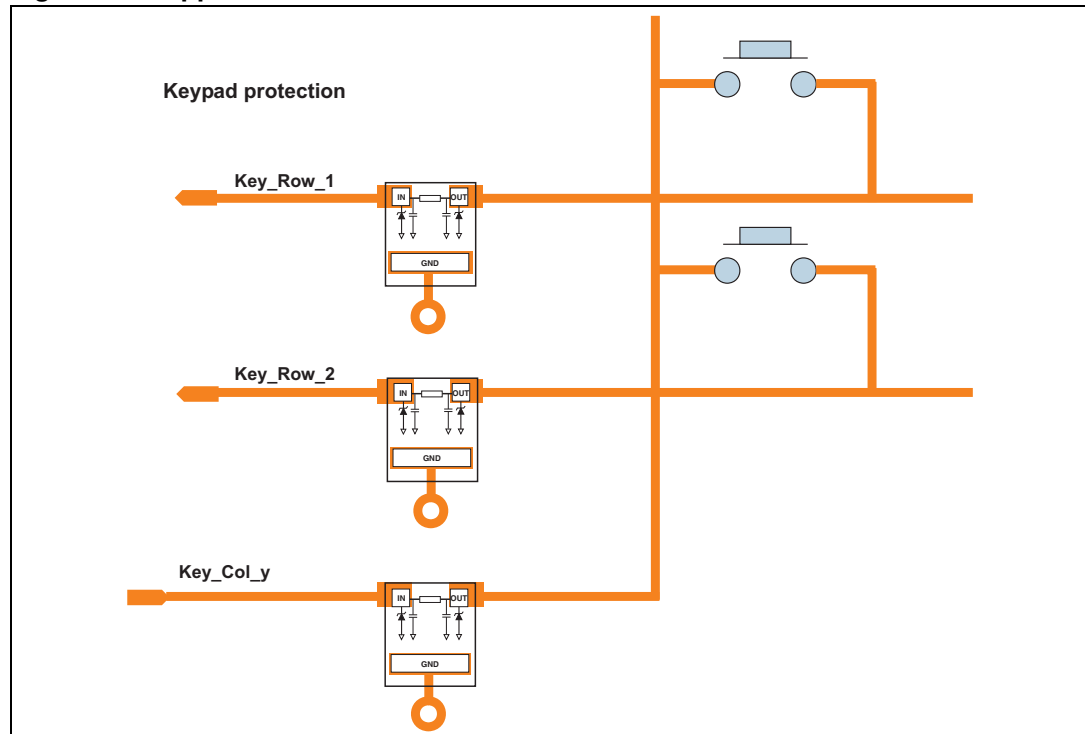
Figure 7. Application schematic
