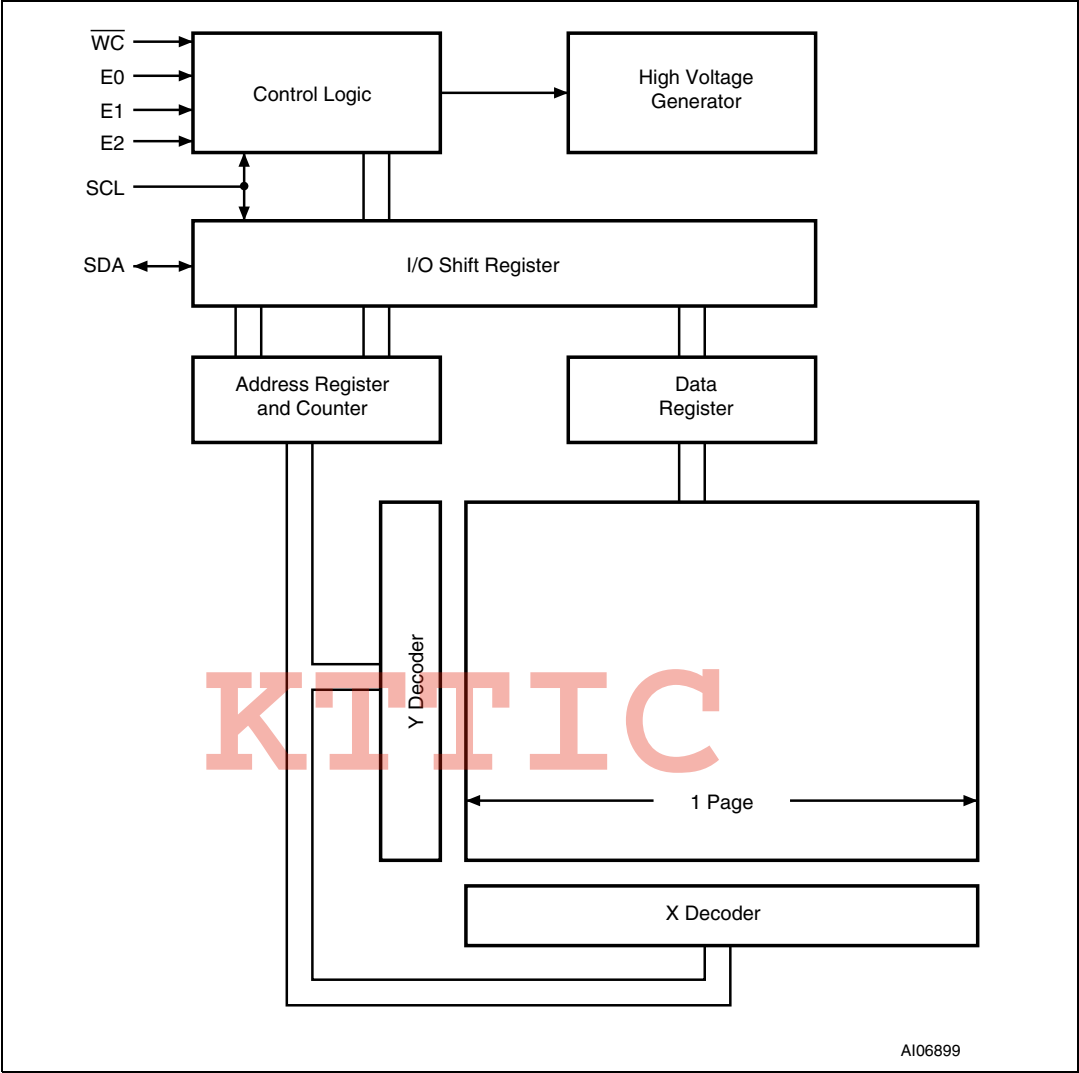
Figure 6. Block diagram
