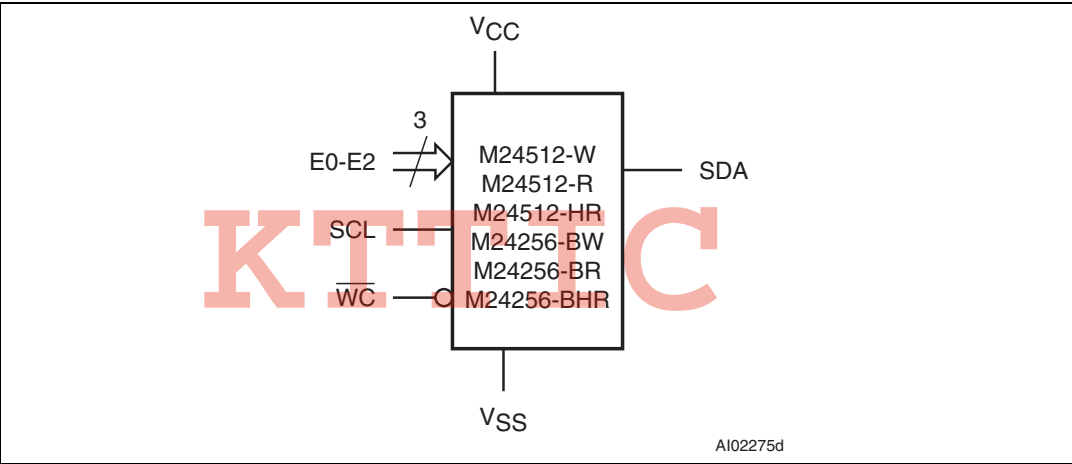
Figure 1. Logic diagram
