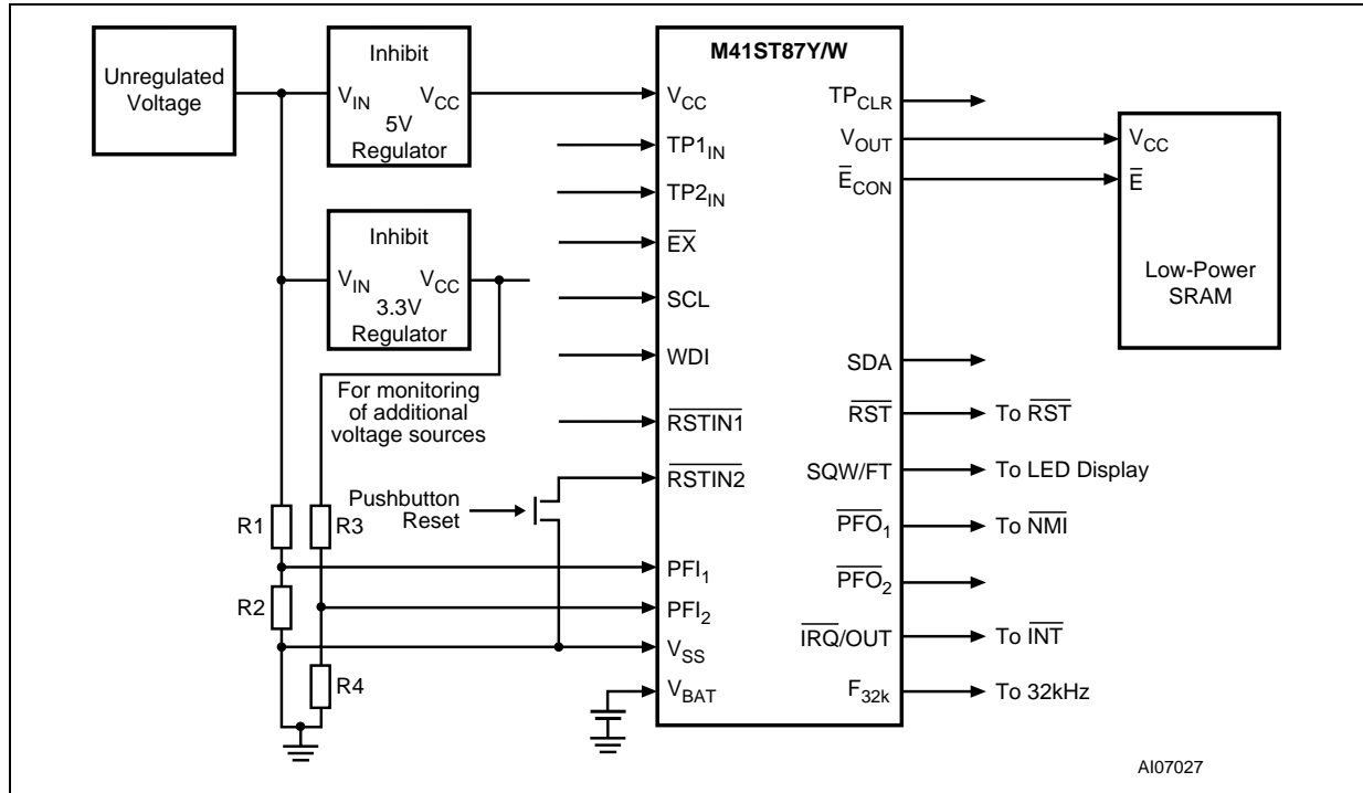
Figure 5. Hardware Hookup
