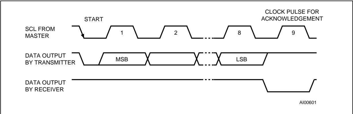
Figure 7. Acknowledgement Sequence
