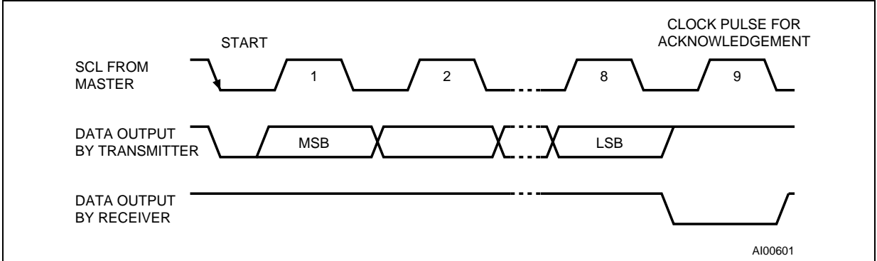
Figure 5. Acknowledgement sequence
