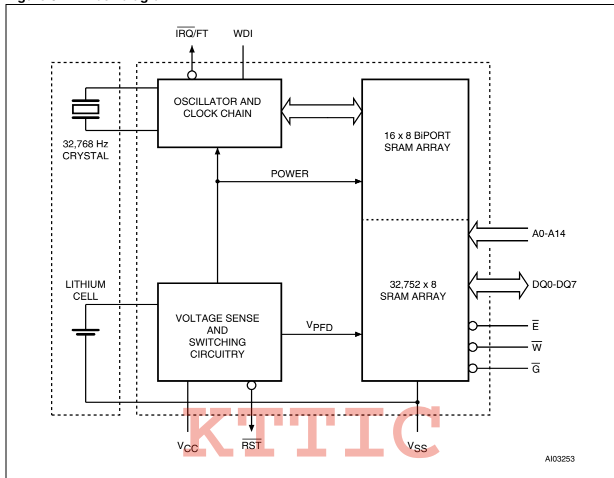
Figure 3. Block diagram
