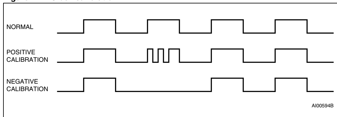
Figure 11. Clock calibration
