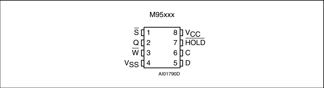
Figure 2. SO connections
