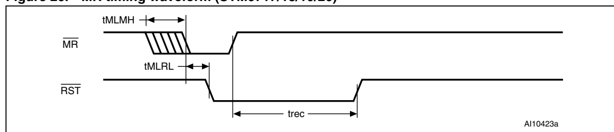
Figure 26. \overline{MR} timing waveform (STM6717/18/19/20)
