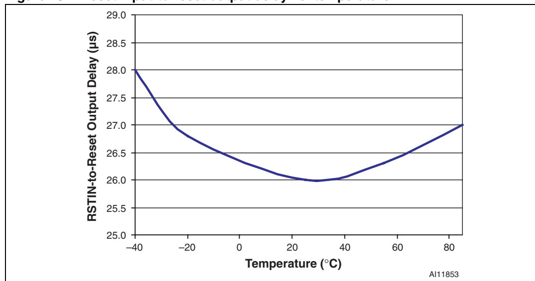
Figure 23. Reset input-to-reset output delay vs. temperature
