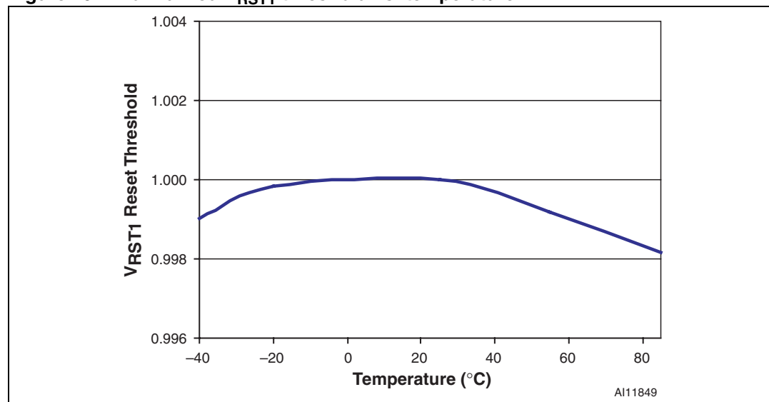
Figure 19. Normalized V_{RST1} threshold vs. temperature
