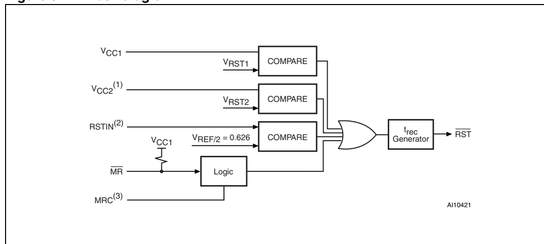
Figure 9. Block diagram
