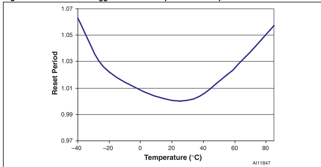
Figure 17. Normalized V_{CC} reset time-out period vs. temperature
