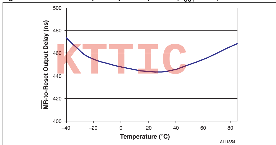
Figure 24. \overline{\text{MR}} -to-reset output delay vs. temperature ( V_{CC1} = 3.6\text{V} )
