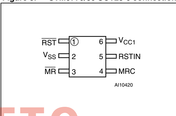
Figure 8. STM6779/80 SOT23-6 connections
