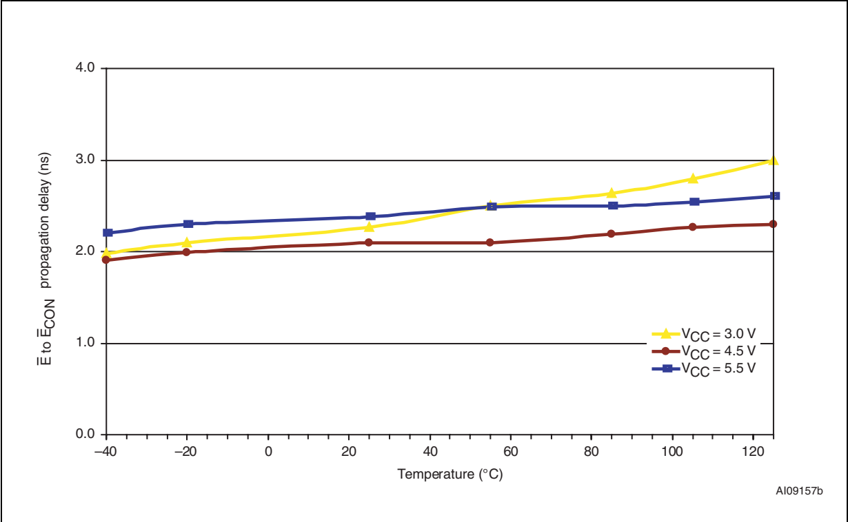
Figure 33. \overline{E} to \overline{E}_{CON} propagation delay vs. temperature
