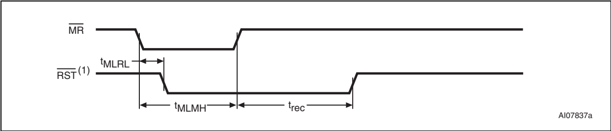
Figure 36. MR timing waveform
