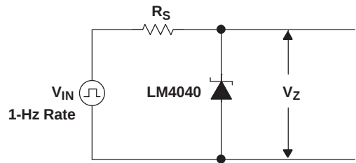
Figure 7. Test Circuit
