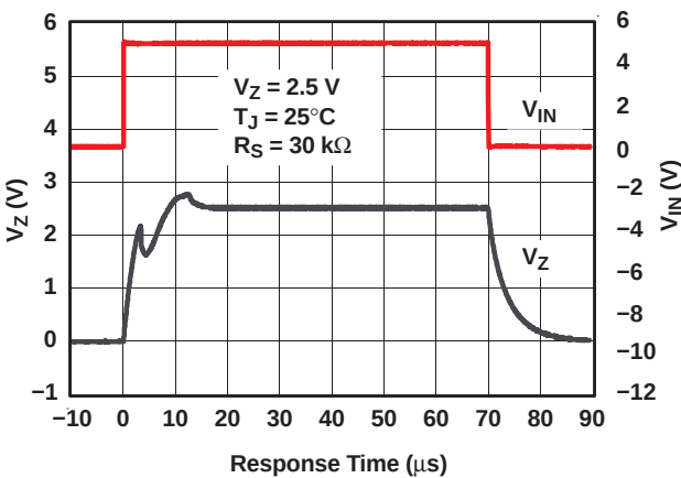
Figure 6. Start-Up Characteristics
