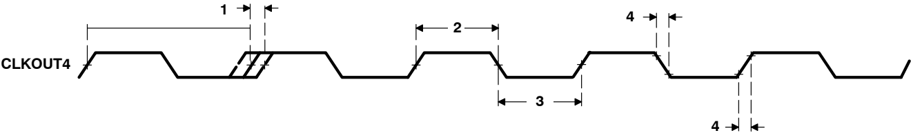
Figure 17. CLKOUT4 Timing
