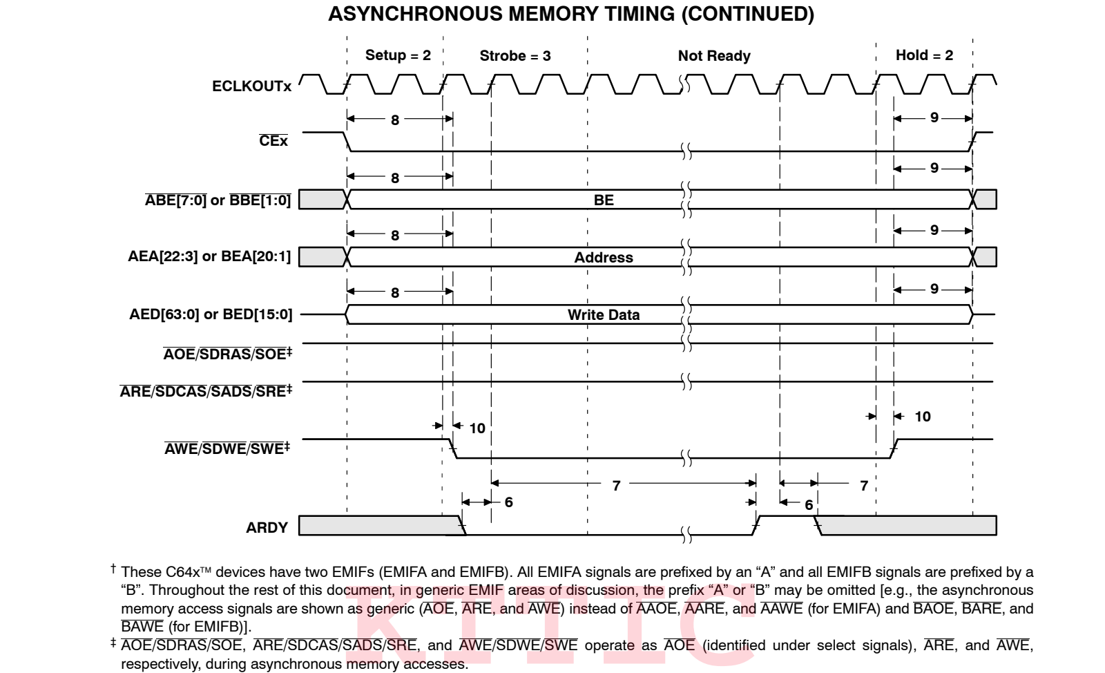
Figure 23. Asynchronous Memory Write Timing for EMIFA and EMIFB†
