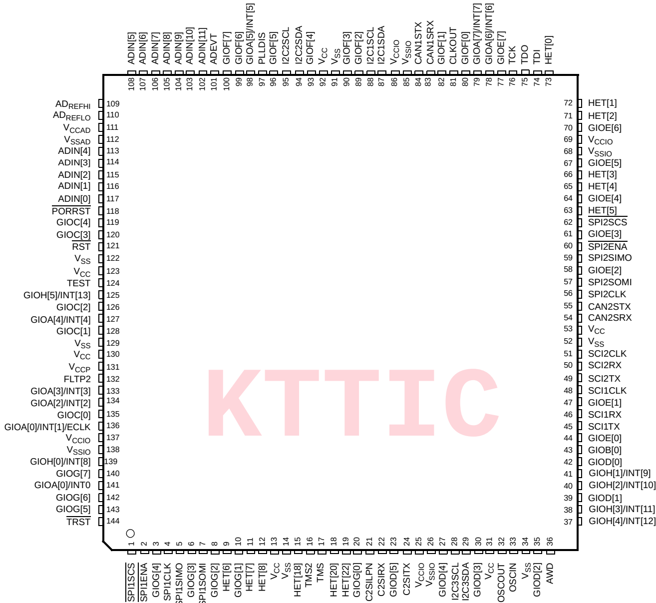
TMS470R1VF288 144-PIN PGE PACKAGE (TOP VIEW) (without Expansion Bus)
