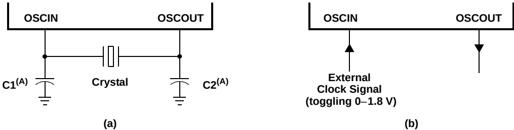
Figure 5. Crystal/Clock Connection
