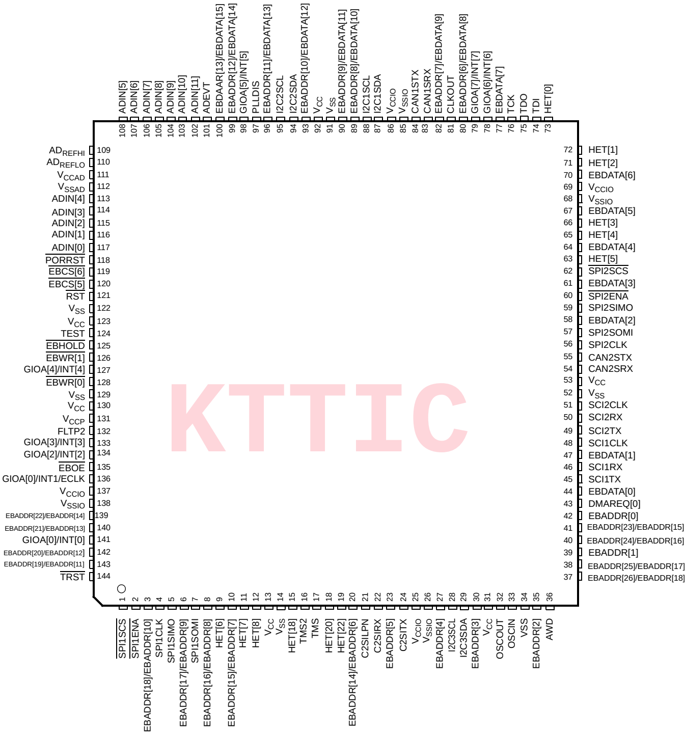
TMS470R1VF288 144-PIN PGE PACKAGE (TOP VIEW) (with Expansion Bus)
