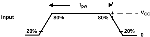
Figure 11. CMOS-Level Inputs
