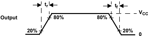
Figure 9. CMOS-Level Outputs
