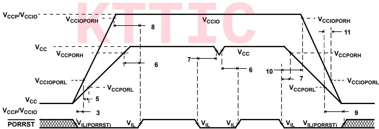
Figure 7. PORRST Timing Diagram
