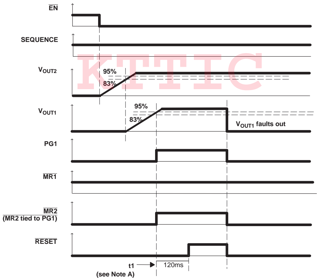
Figure 43. Timing when V_{\text{OUT1}} Faults Out
