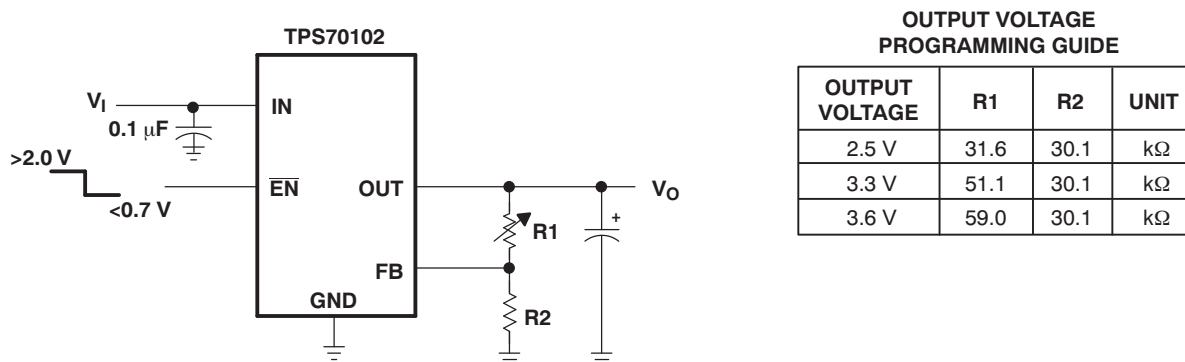
Figure 50. TPS70102 Adjustable LDO Regulator Programming
