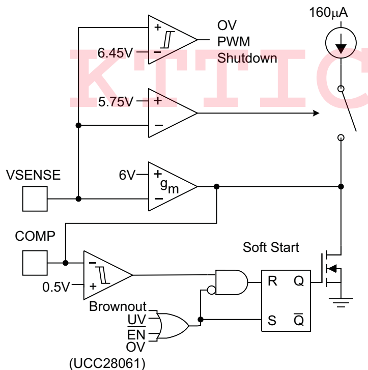
Figure 29. Error Amplifier Block Diagram Showing Speed-Up and Latched Soft-Start
