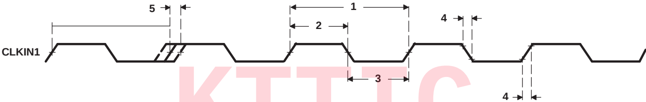
Figure 7-21. CLKIN1 Timing
