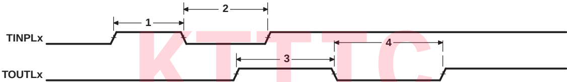
Figure 7-73. Timer Timing
