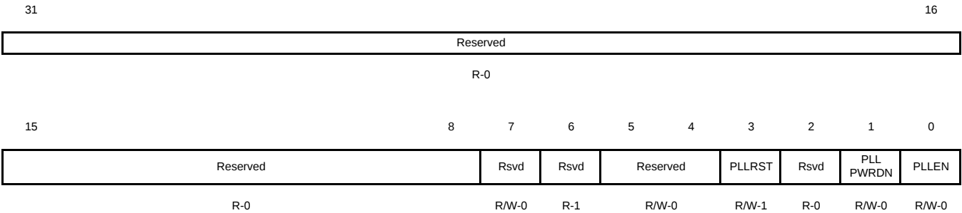
Figure 7-11. PLL1 Control Register (PLLCTL) [Hex Address: 029A 0100]
