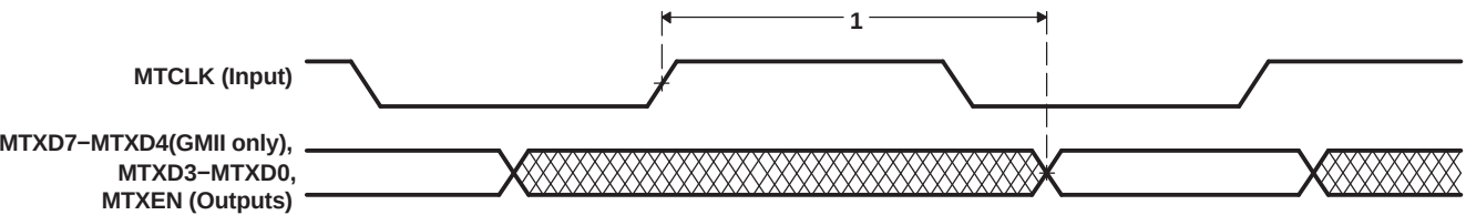
Figure 7-63. EMAC Transmit Interface Timing [MII and GMII Operation]
