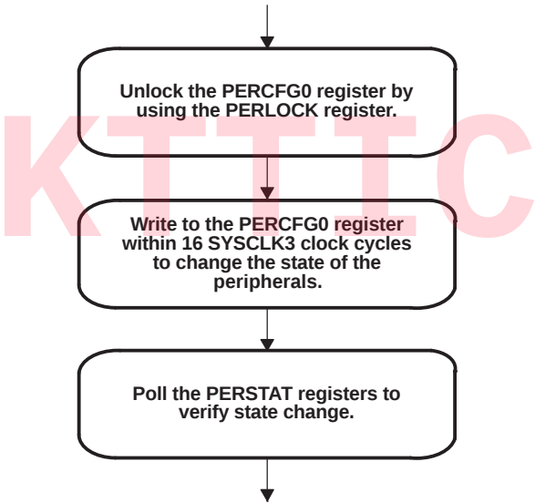
Figure 3-2. Peripheral State Change Flow
