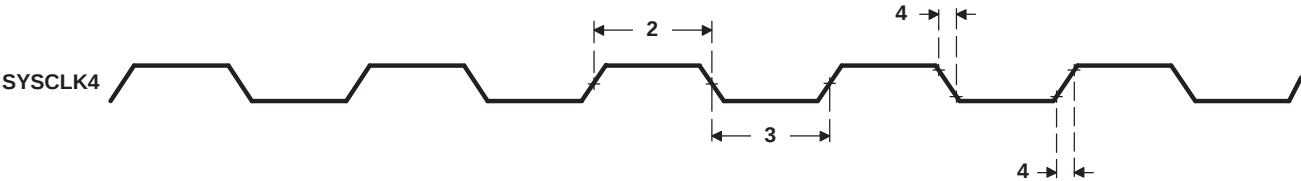
Figure 7-22. SYSCLK4 Timing
