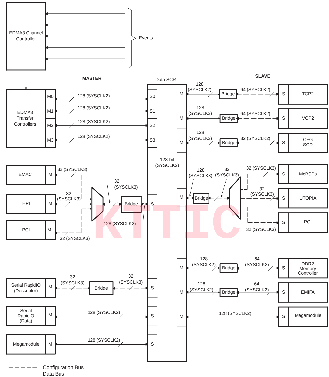
Figure 4-1. Switched Central Resource Block Diagram
