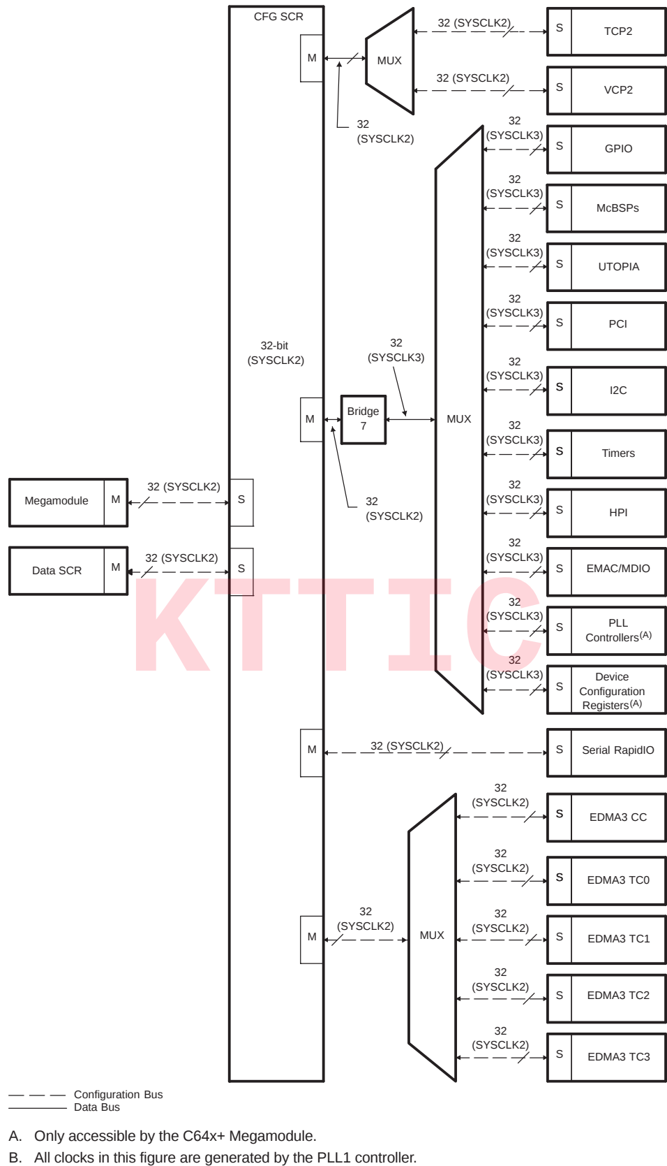
Figure 4-2. C64x+ Megamodule - SCR Connection
