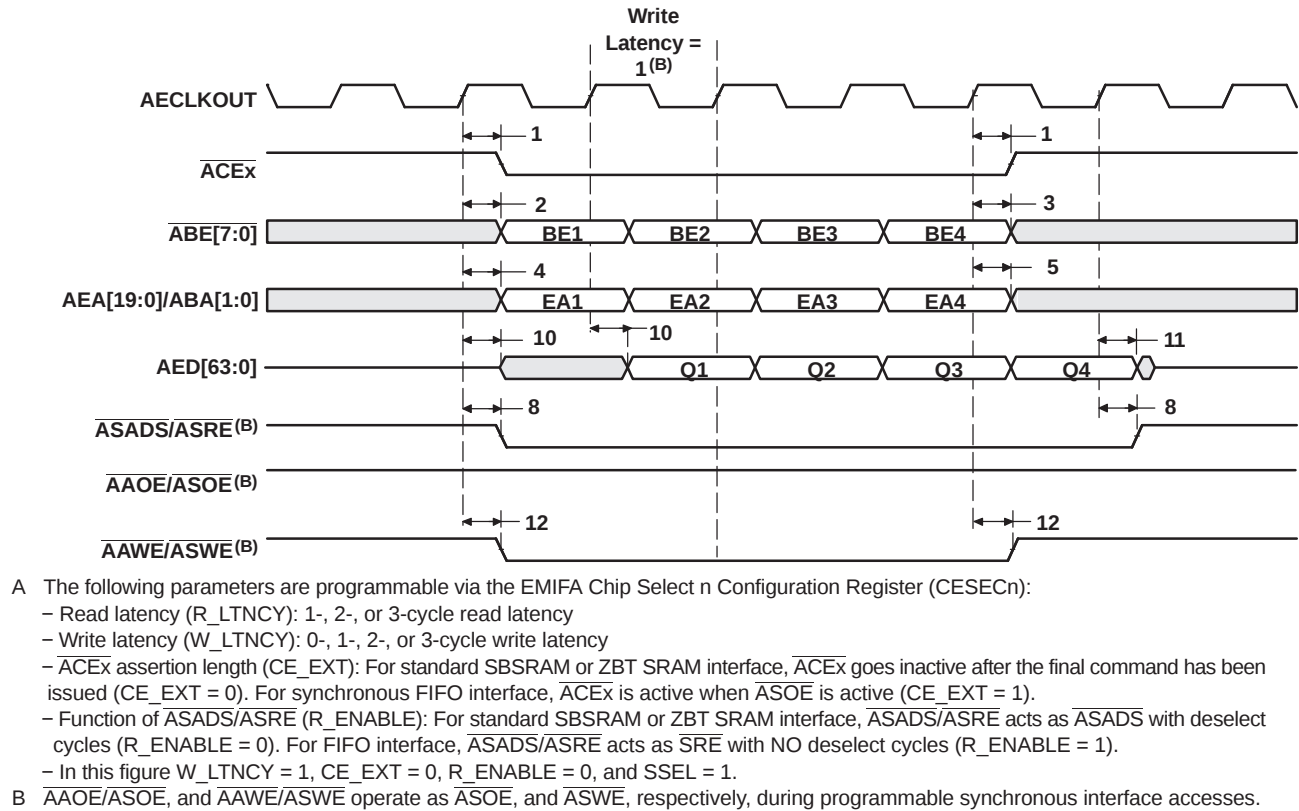
Figure 7-38. Programmable Synchronous Interface Write Timing for EMIFA (With Write Latency = 1) (A)
