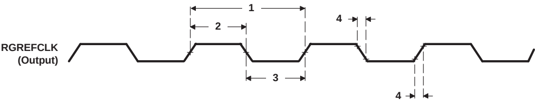
Figure 7-68. RGMIIREFCLK Timing
