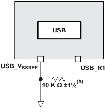
Figure 6-42. USB Reference Resistor Routing
