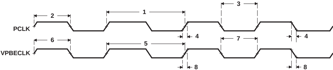
Figure 6-32. VPBE PCLK and VPBECLK Timing
