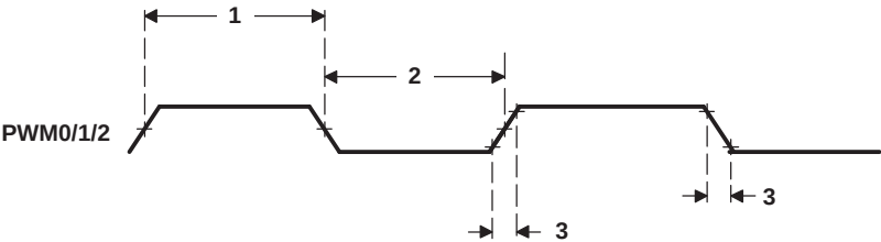
Figure 6-57. PWM Output Timing
