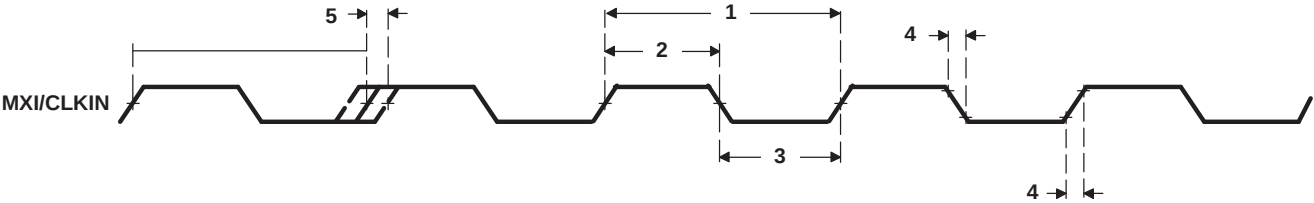
Figure 6-13. MXI/CLKIN Timing
