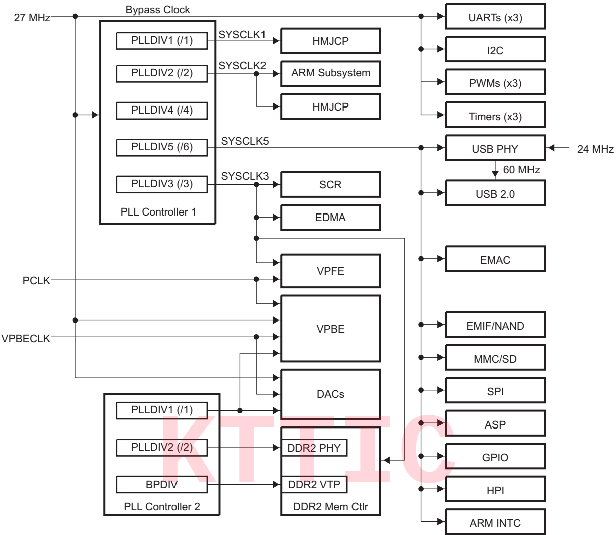
Figure 6-5. PLL1 and PLL2 Clock Domain Block Diagram
