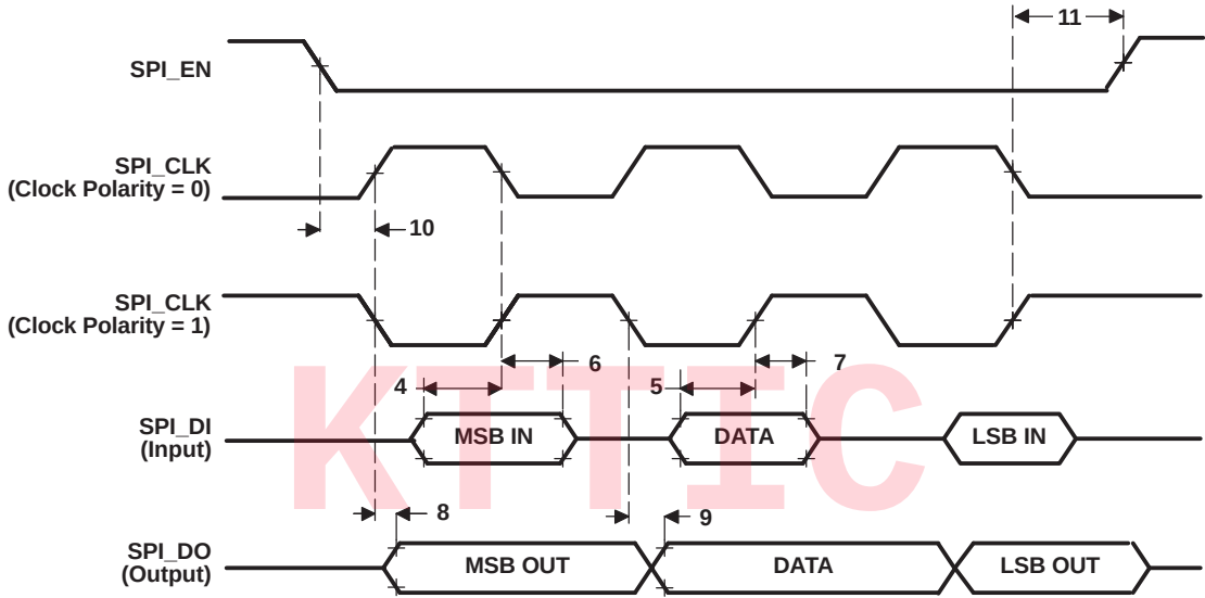
Figure 6-45. SPI Master Mode External Timing (Clock Phase = 0)
