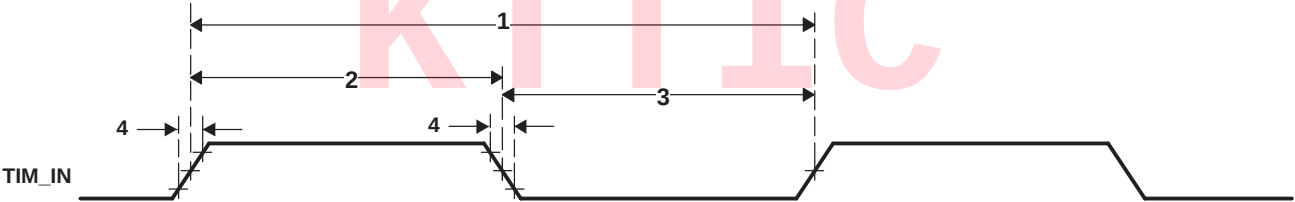
Figure 6-56. Timer Timing
