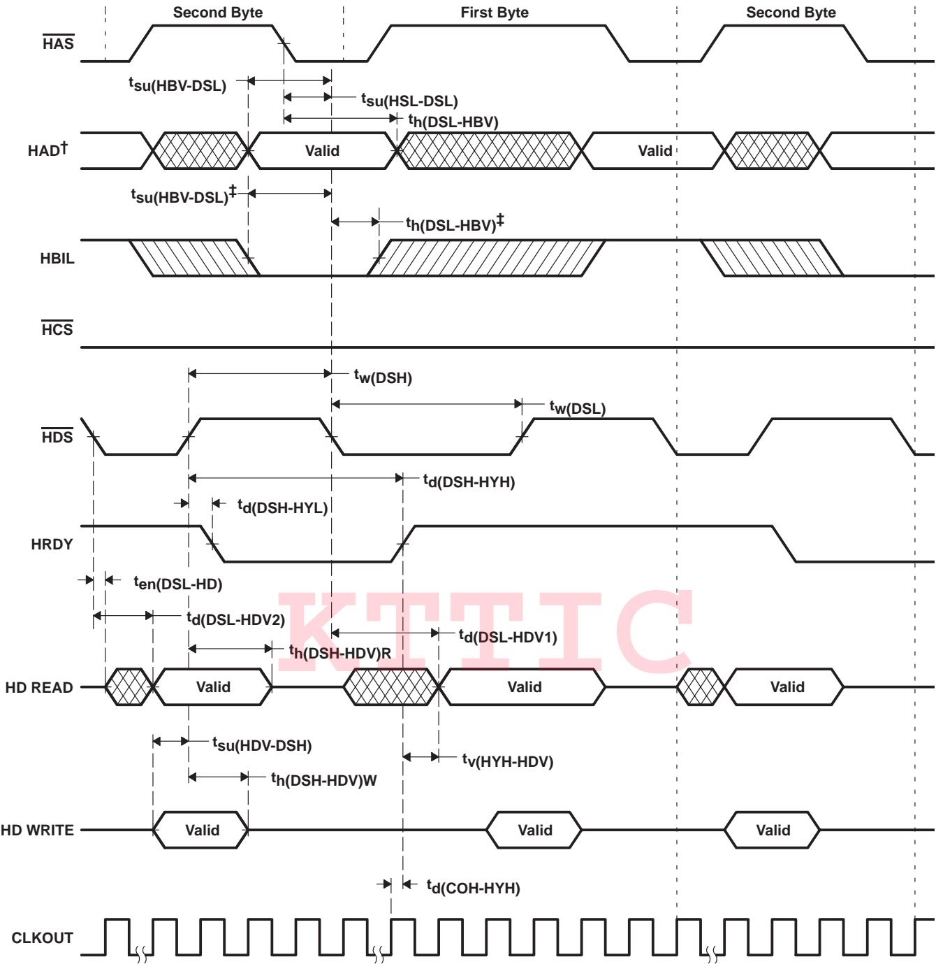
Figure 4-27. Using HDS to Control Accesses (HCS Always Low)
