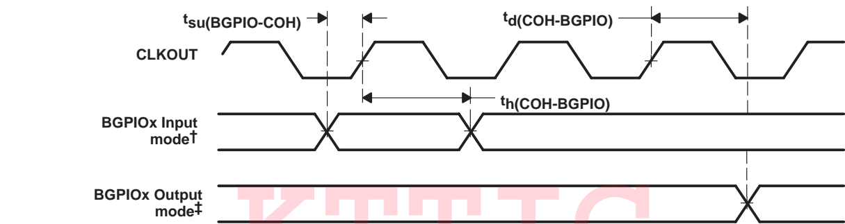
Figure 4–22. McBSP General-Purpose I/O Timings
