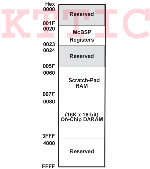
Figure 2-9. UC5402 DMA Memory Map
