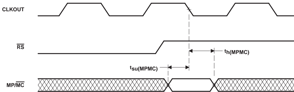
Figure 4–16. \overline{\text{MP/MC}} Timing
