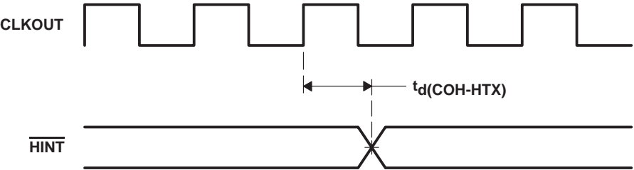
Figure 4–29. \overline{\text{HINT}} Timing
