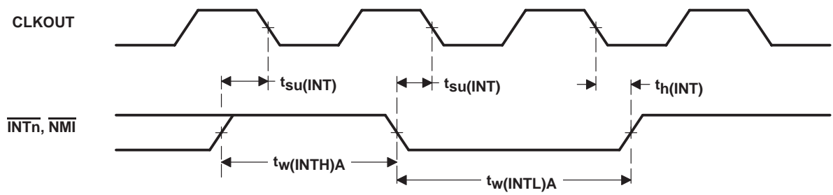
Figure 4–15. Interrupt Timing
