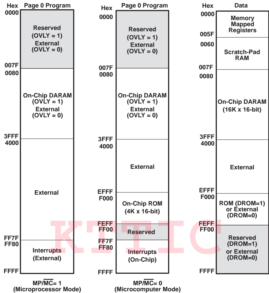
Figure 2-2. TMS320UC5402 Memory Map
