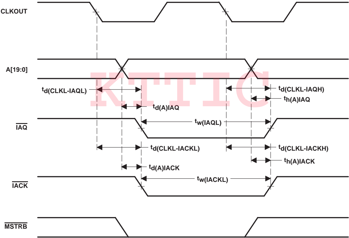
Figure 4–17. \overline{\text{IAQ}} and \overline{\text{IACK}} Timings
