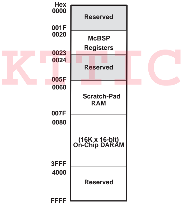
Figure 2–8. UC5402 HPI8 Memory Map
