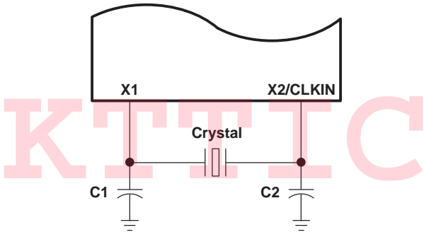
Figure 5-2. Internal Divide-By-Two Clock Option With External Crystal
