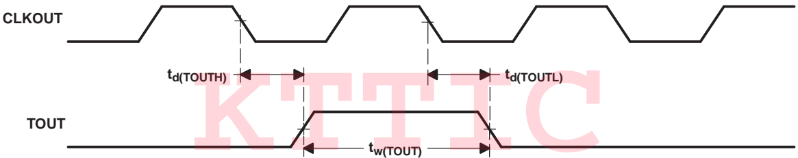
Figure 5-20. TOUT Timing
