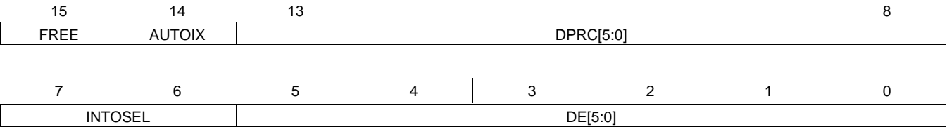
Figure 3-22. DMPREC Register
