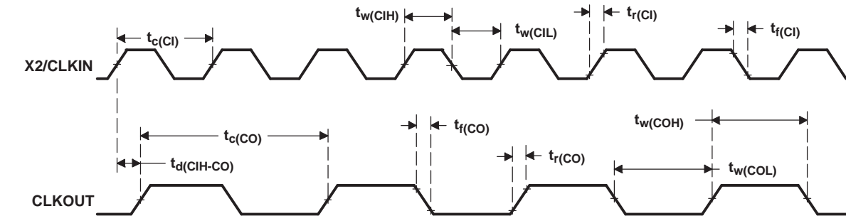
Figure 5-3. External Divide-By-Two Clock Timing
