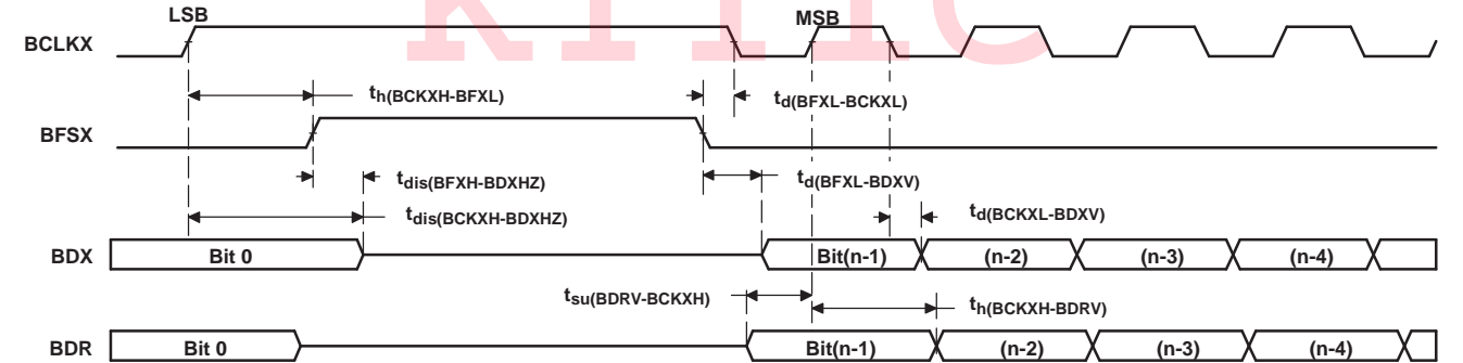
Figure 5-26. McBSP Timing as SPI Master or Slave: CLKSTP = 10b, CLKXP = 1
